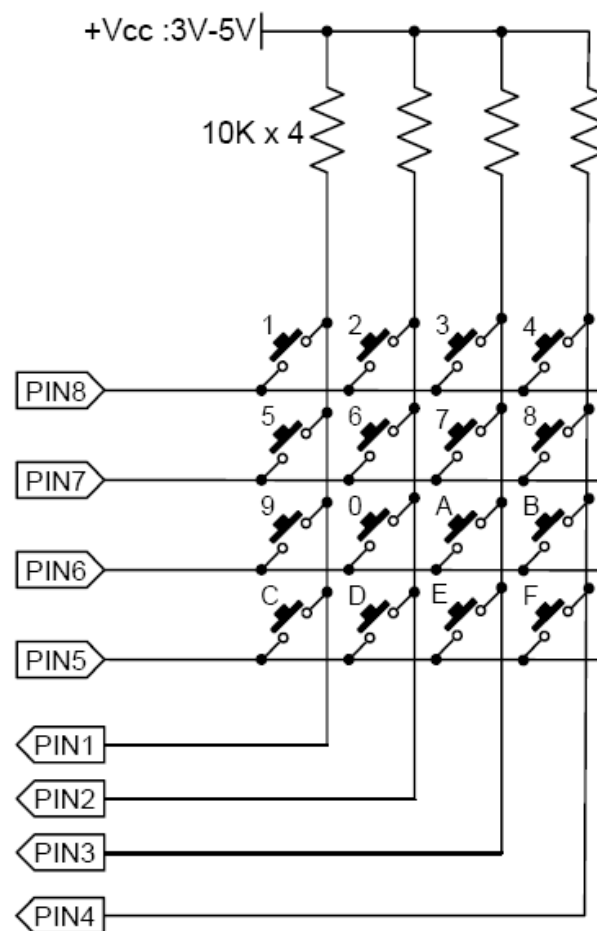
FIG 3: MR-MINI-4x4KEY Schematic
