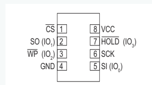
Figure 2-2. 8-UDFN — Top View
