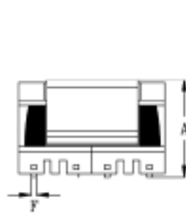
Figure 10. FT-X3 Dimensions
