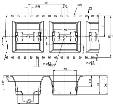
Figure 14. FT-X3 Reel and Tape Device Placement
