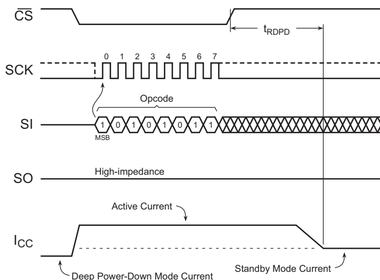
Figure 7-2. Resume from Deep Power-Down
