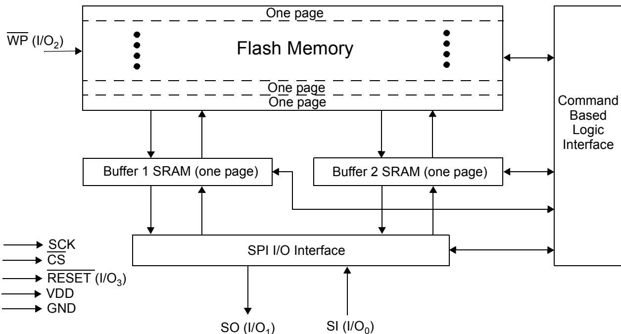
Figure 2-1. Block Diagram of the AT45DB321F Device
