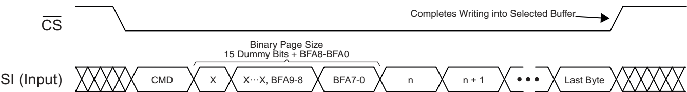
Figure 20-1. Buffer Write
