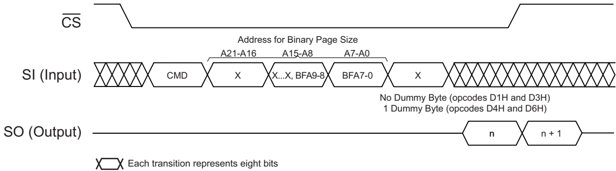
Figure 21-3. Buffer Read
