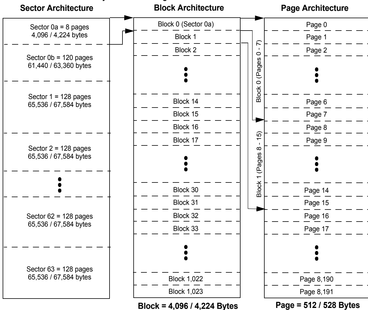
Figure 3-1. AT45DB321F Memory Architecture Diagram
