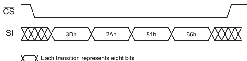
Figure 4-3. Quad Enable
