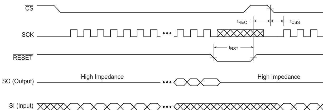
Figure 22-11. Reset Timing
