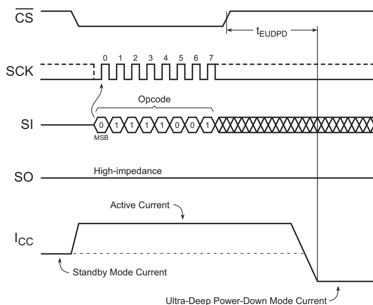
Figure 7-3. Ultra-Deep Power-Down
