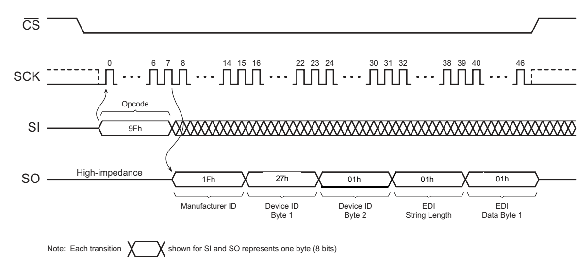
Figure 9-1. Read Manufacturer and Device ID
