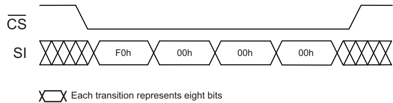
Figure 10-1. Software Reset
