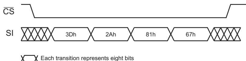
Figure 4-4. Quad Disable
