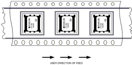
Figure 19: FT-X3 Device Placement on the Carrier Tape
