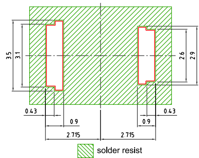
Component Location on Pad
