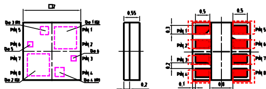
Component Location on Pad
