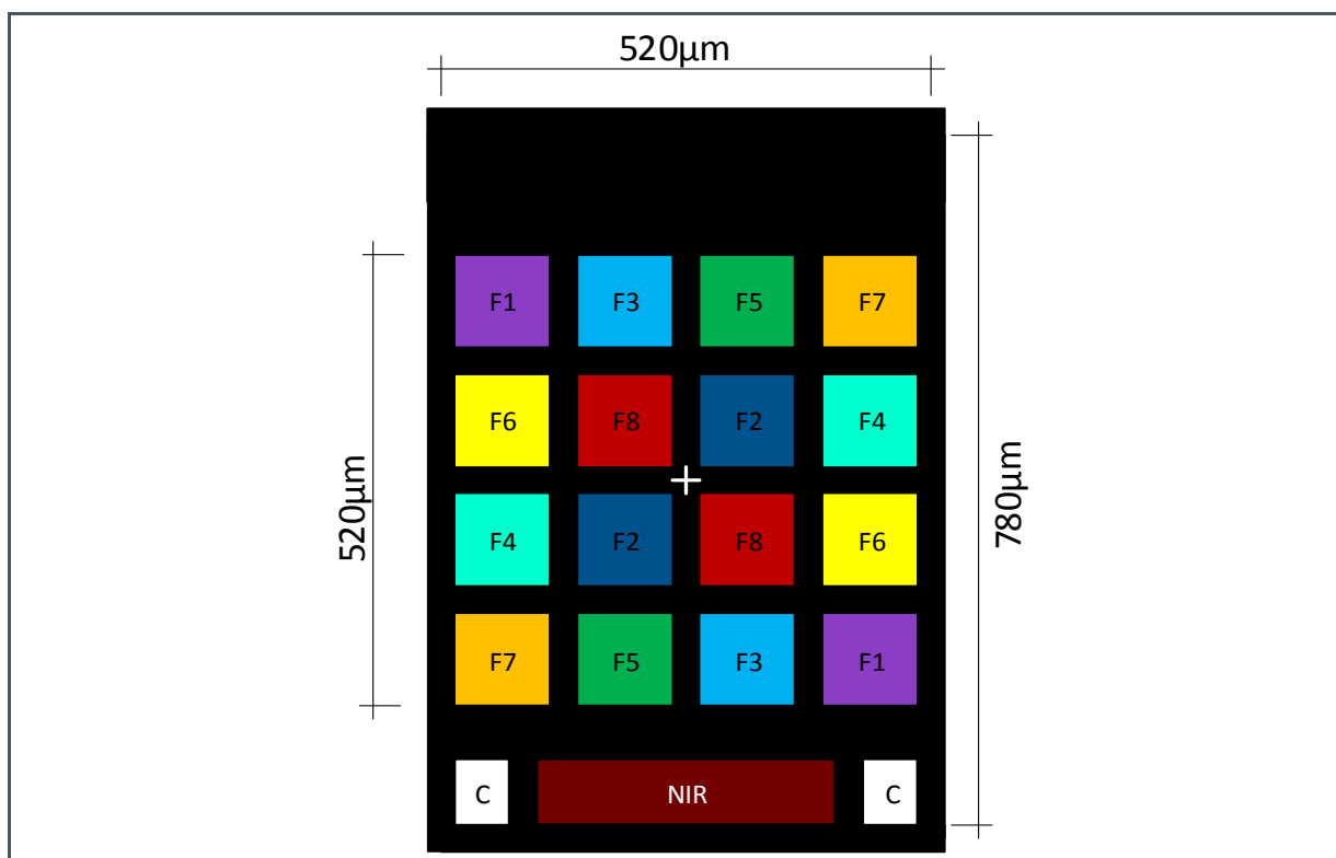
Figure 21: Sensor Array
