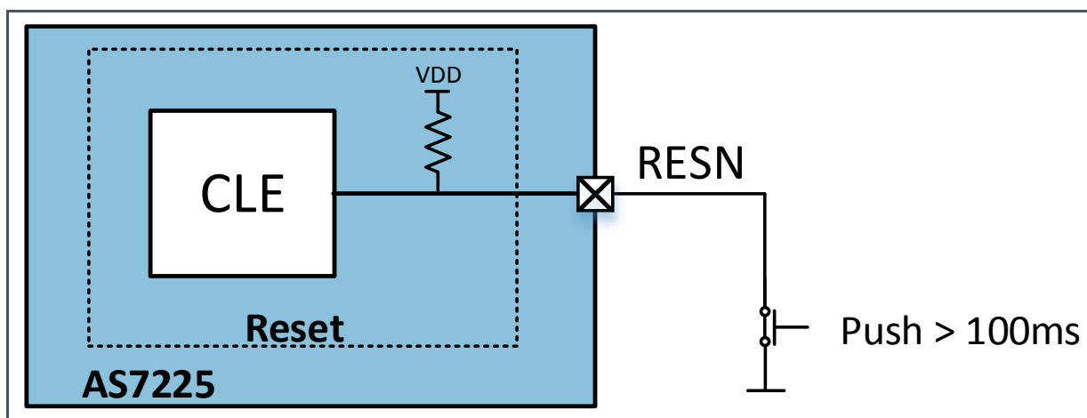
Figure 12: Reset Circuit
