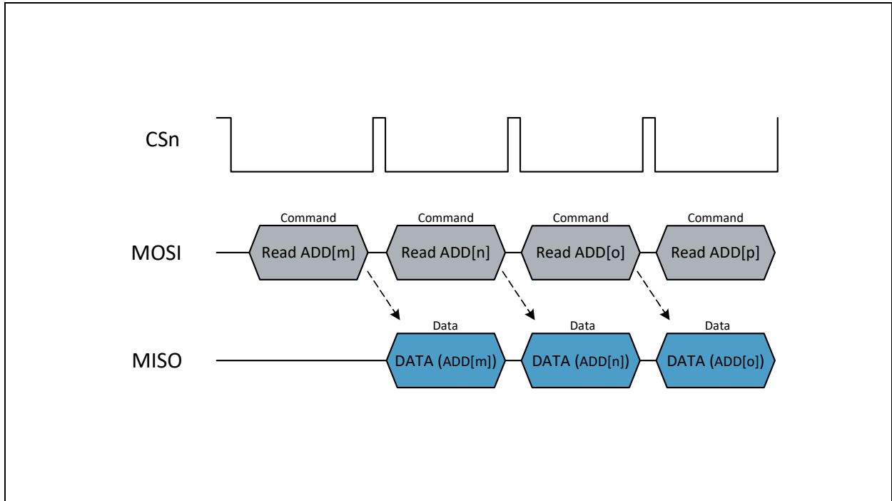
Figure 31: SPI Read
