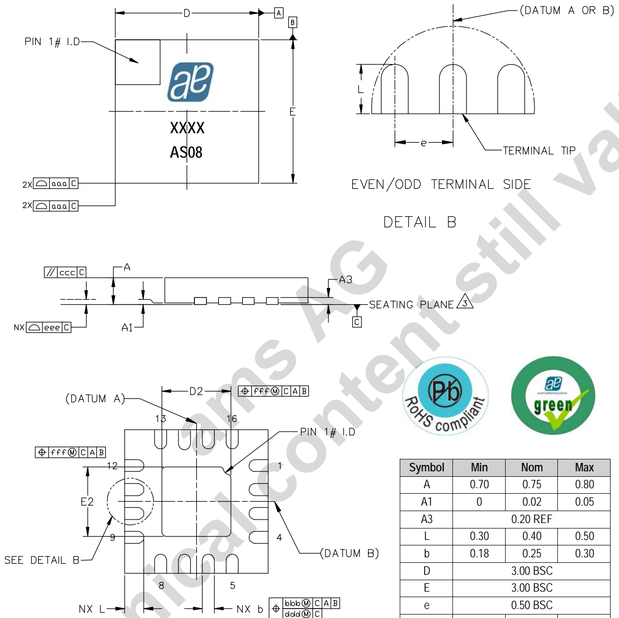
Figure 29. TQFN-16 (3x3mm)
