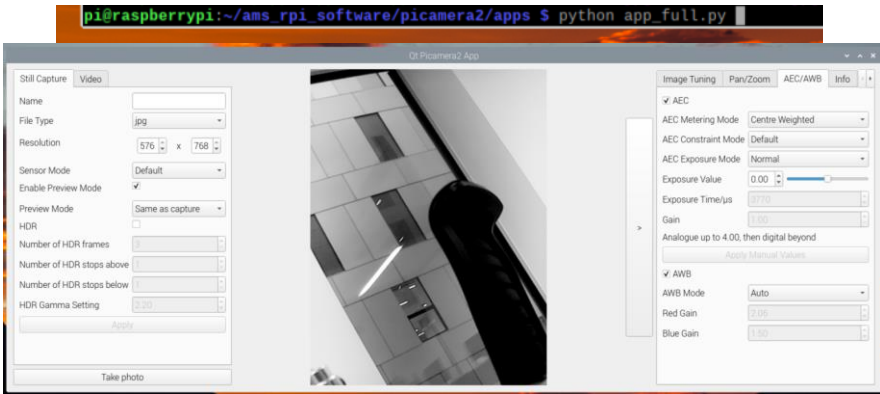
Figure 9: App_full.py
