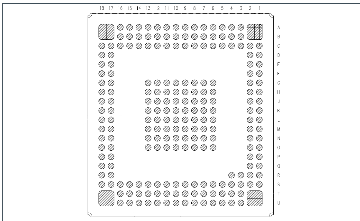
Figure 3: Pin Diagram
