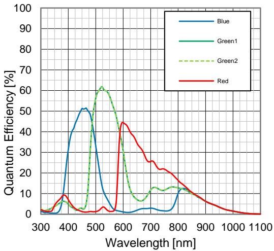
Figure 10: Quantum Efficiency Color
