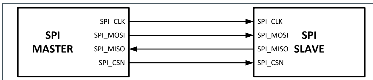
Figure 19: SPI Connection Diagram
