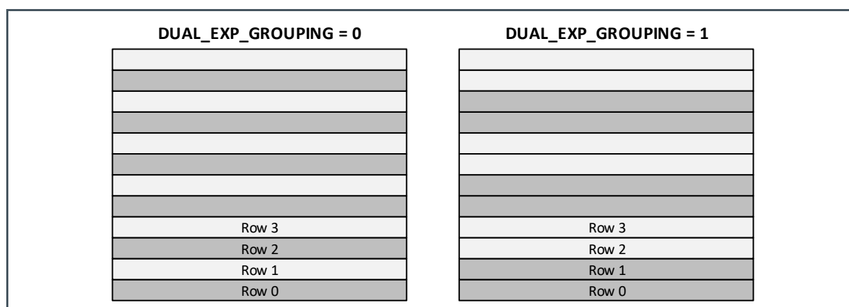
Figure 89: Dual Exposure Grouping
