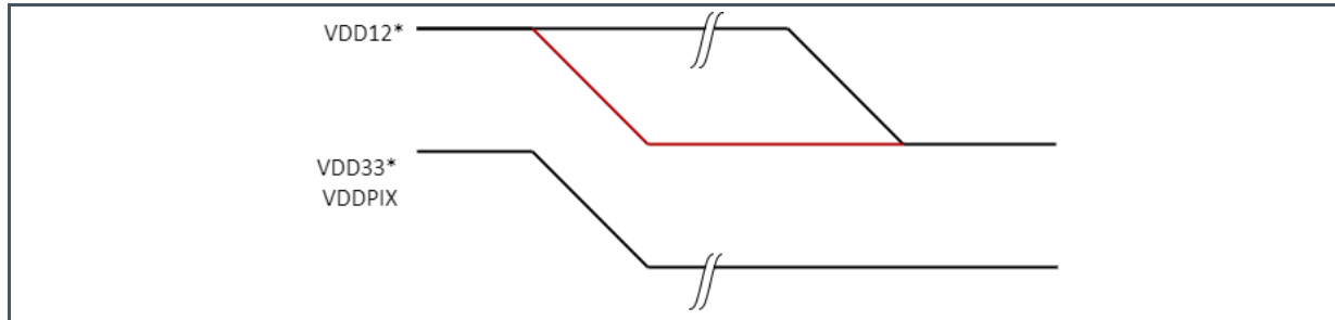
Figure 66: Power-Down Sequence
