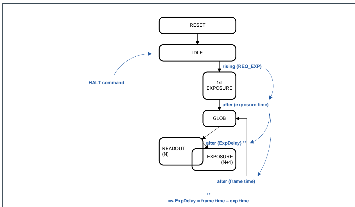
Figure 50: State Diagram: Streaming Mode
