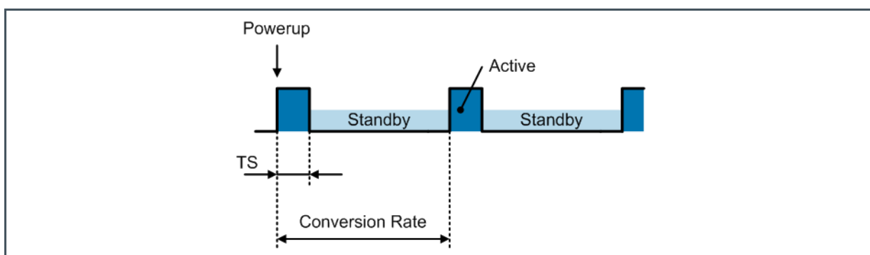
Figure 17: Conversion Sequence
