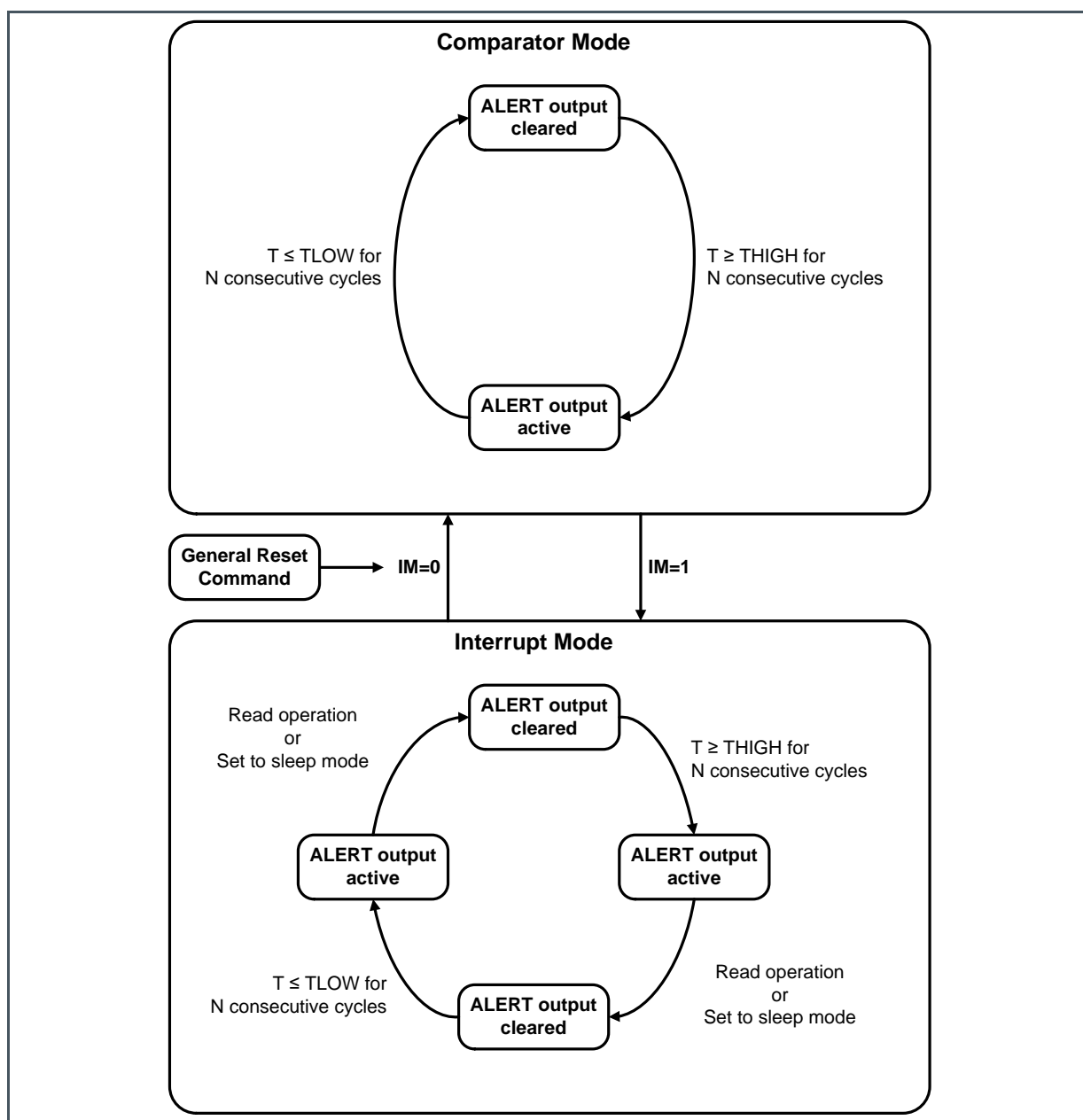
Figure 24: Alert Operation Modes
