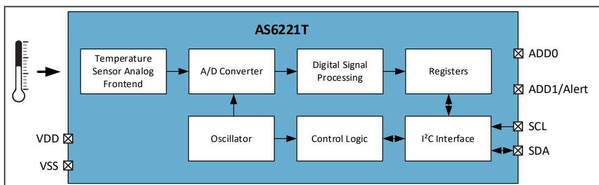
Figure 2 : Functional Blocks of AS6221T
