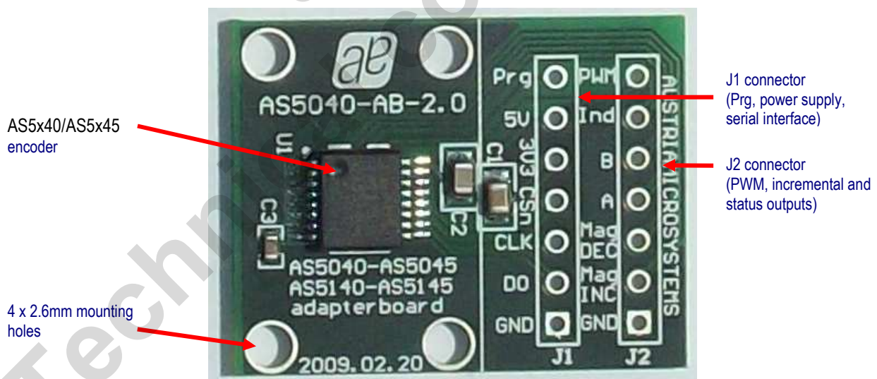
Figure 1: AS5040 Adapterboard
