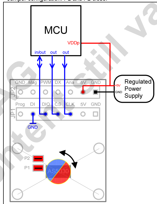
Figure 8: Bidirectional serial connection (3 wire)
