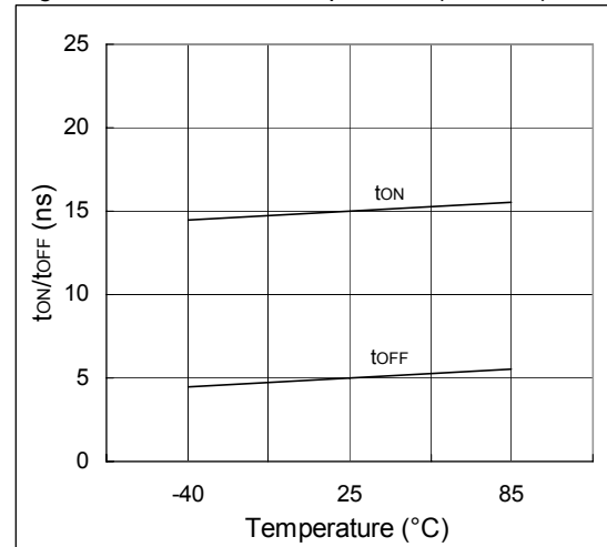
Figure 8. t_{ON}/t_{OFF} vs. Temperature ( V_{+} = 5V )
