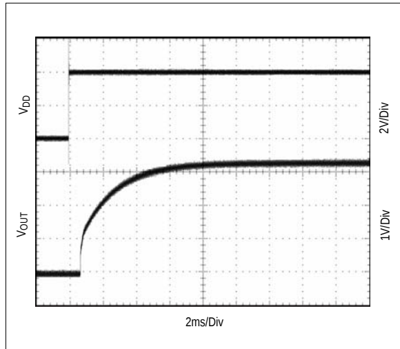
Figure 9. Startup; no Load, C_{REF} = 100\text{nF}
