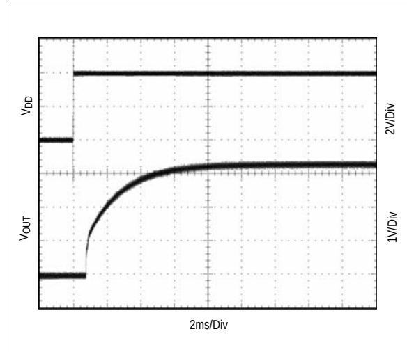
Figure 10. Startup; R_{LOAD} = 11\Omega , C_{REF} = 100\text{nF}
