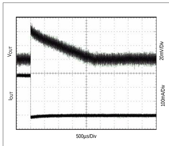
Figure 14. Load Transient Response; I_{OUT} = 300 to 0\text{mA}
