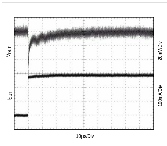
Figure 13. Load Transient Response; I_{OUT} = 0 to 300\text{mA}
