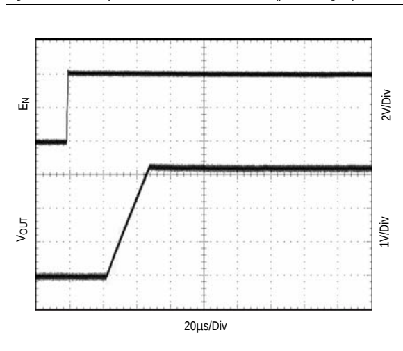
Figure 11. Startup; no Load, C_{REF} = 100\text{nF} (pre-charged)
