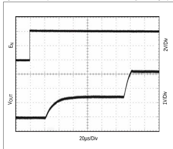
Figure 12. Startup; R_{LOAD} = 11\Omega , C_{REF} = 100\text{nF} (pre-charged)
