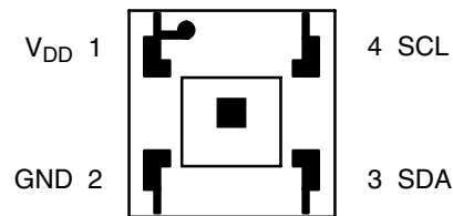
Package Drawing Not to Scale
