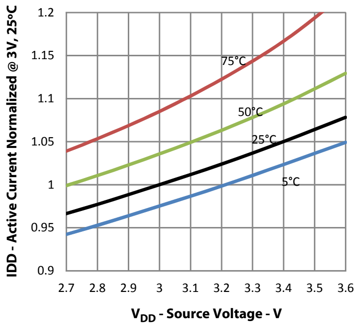
Figure 13: Normalized I_{DD} vs. V_{DD} and Temperature
