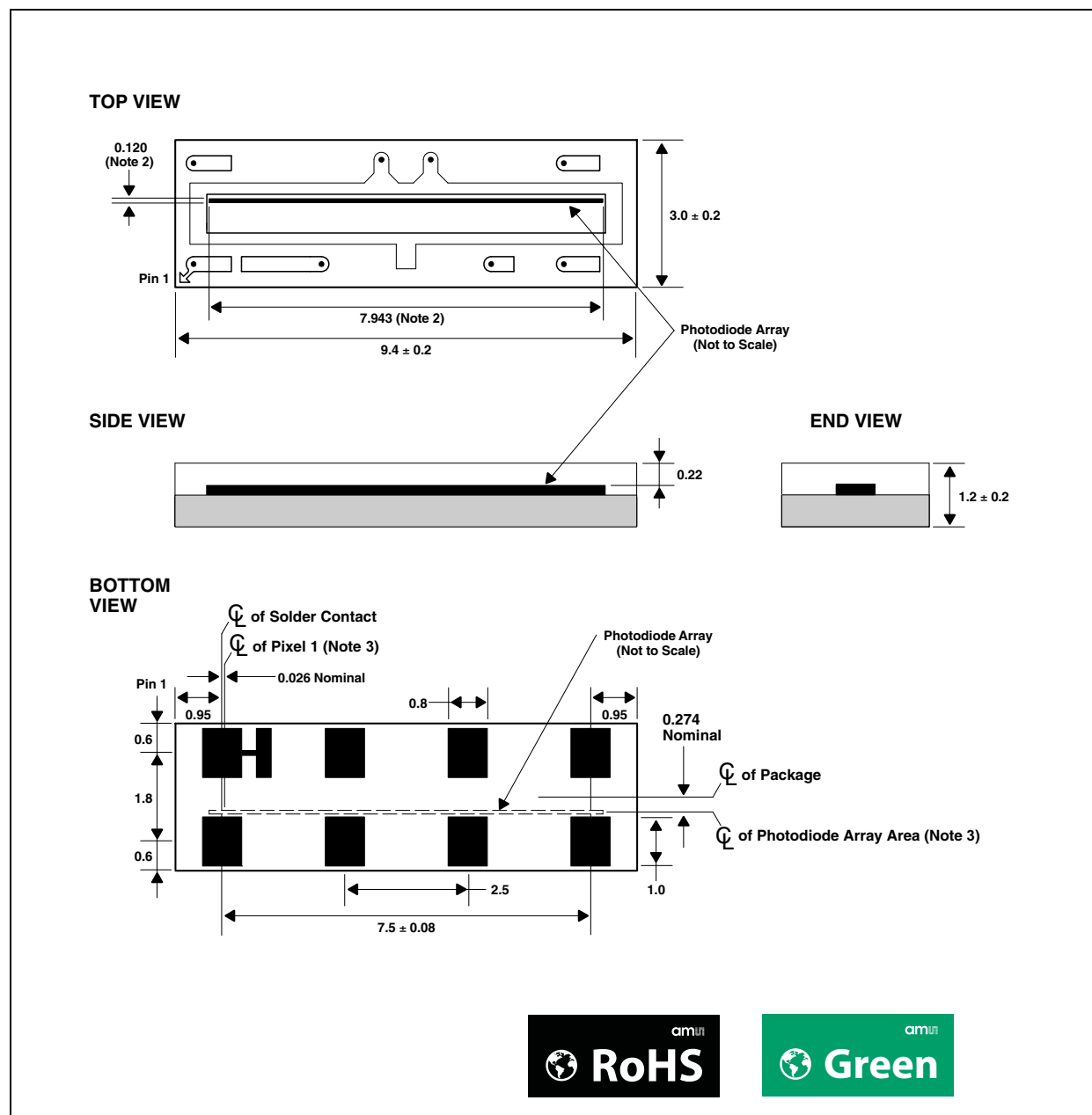
Figure 15: Package CL Configuration
