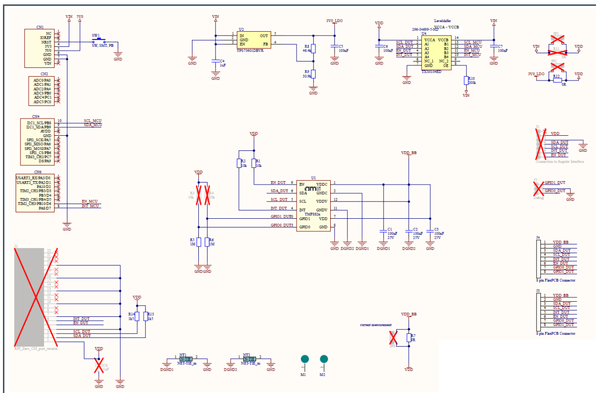
Figure 3: TMF882X-SHIELD Schematic
