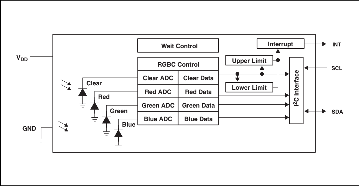
Figure 2: TCS3471 Block Diagram
