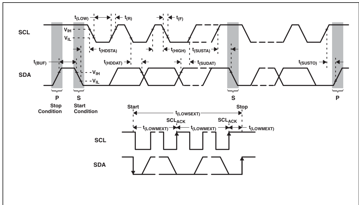
Figure 12: Timing Diagrams
