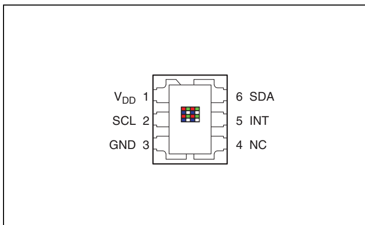
Figure 3: Package FN Dual Flat No-Lead (Top View)
