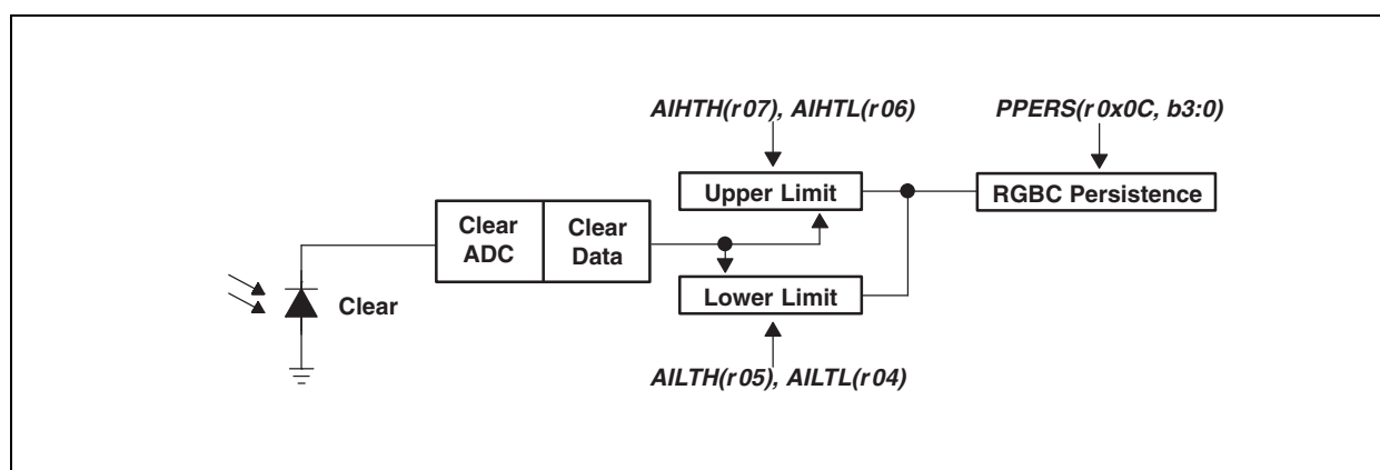
Figure 19: Programmable Interrupt
