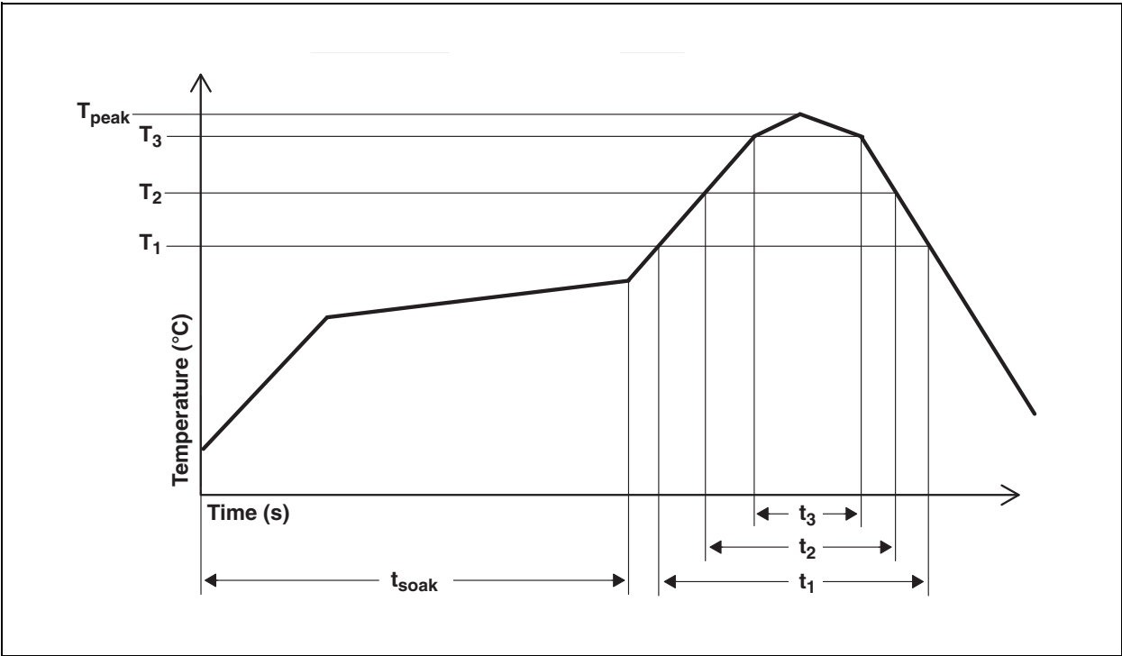
Figure 39: Solder Reflow Profile Graph
