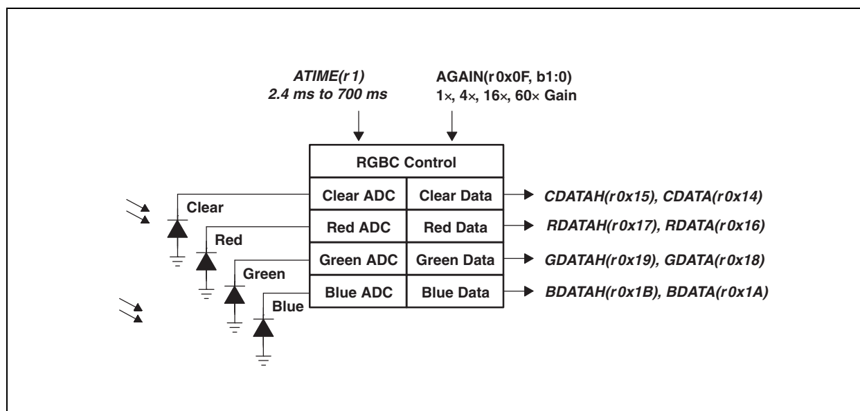
Figure 18: RGBC Operation
