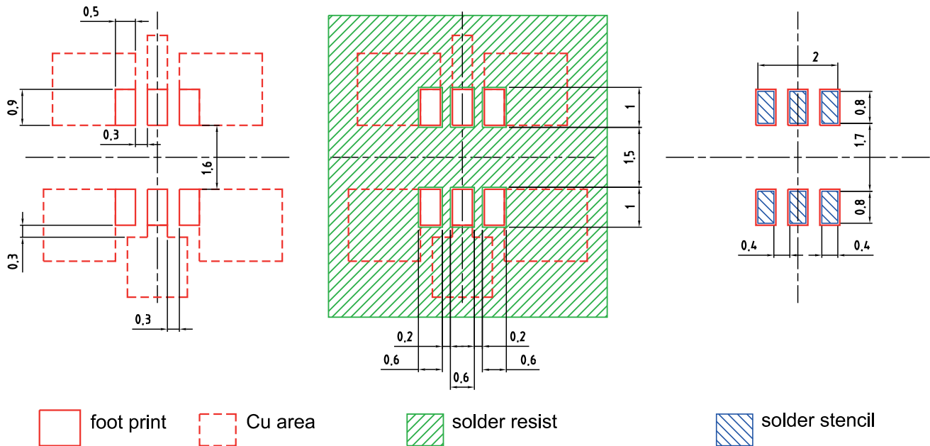
Component Location on Pad
