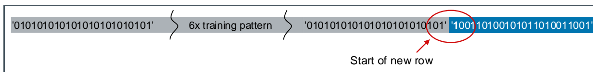
Figure 23 : Start of Row Identification
