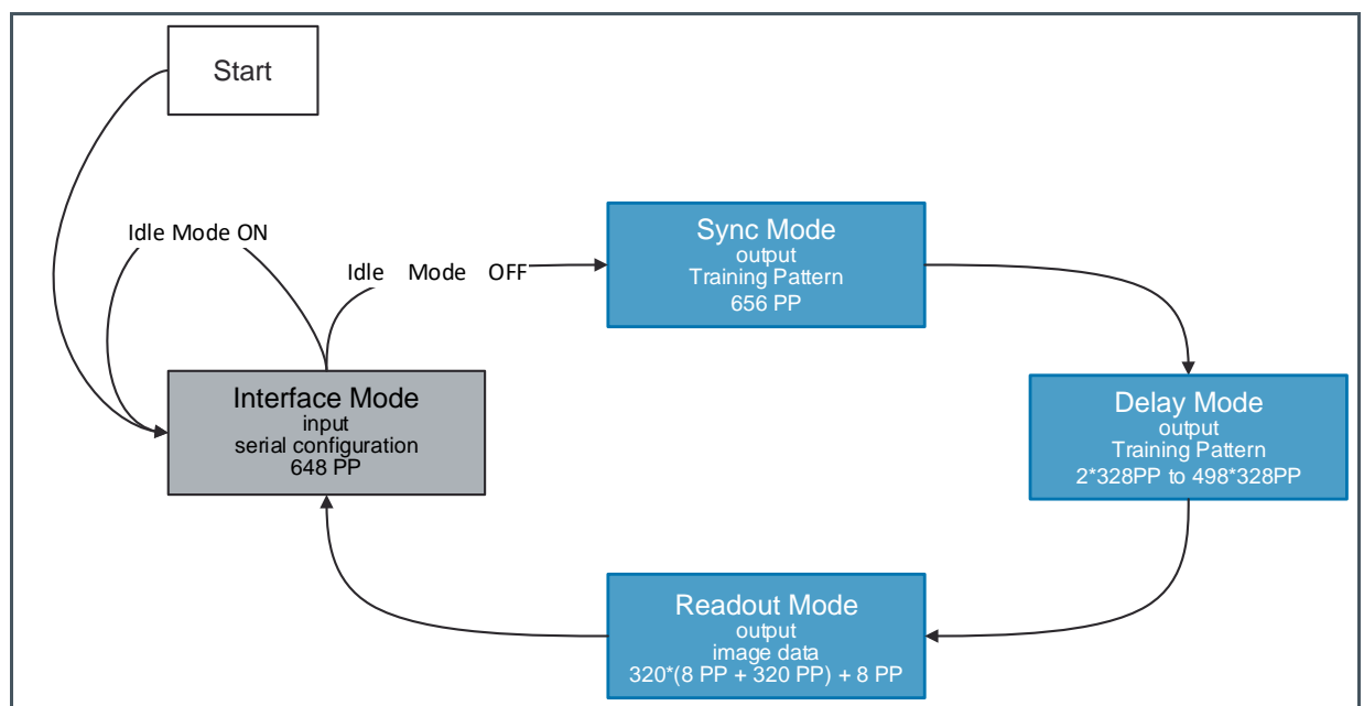
Figure 16: Sequence of Operation
