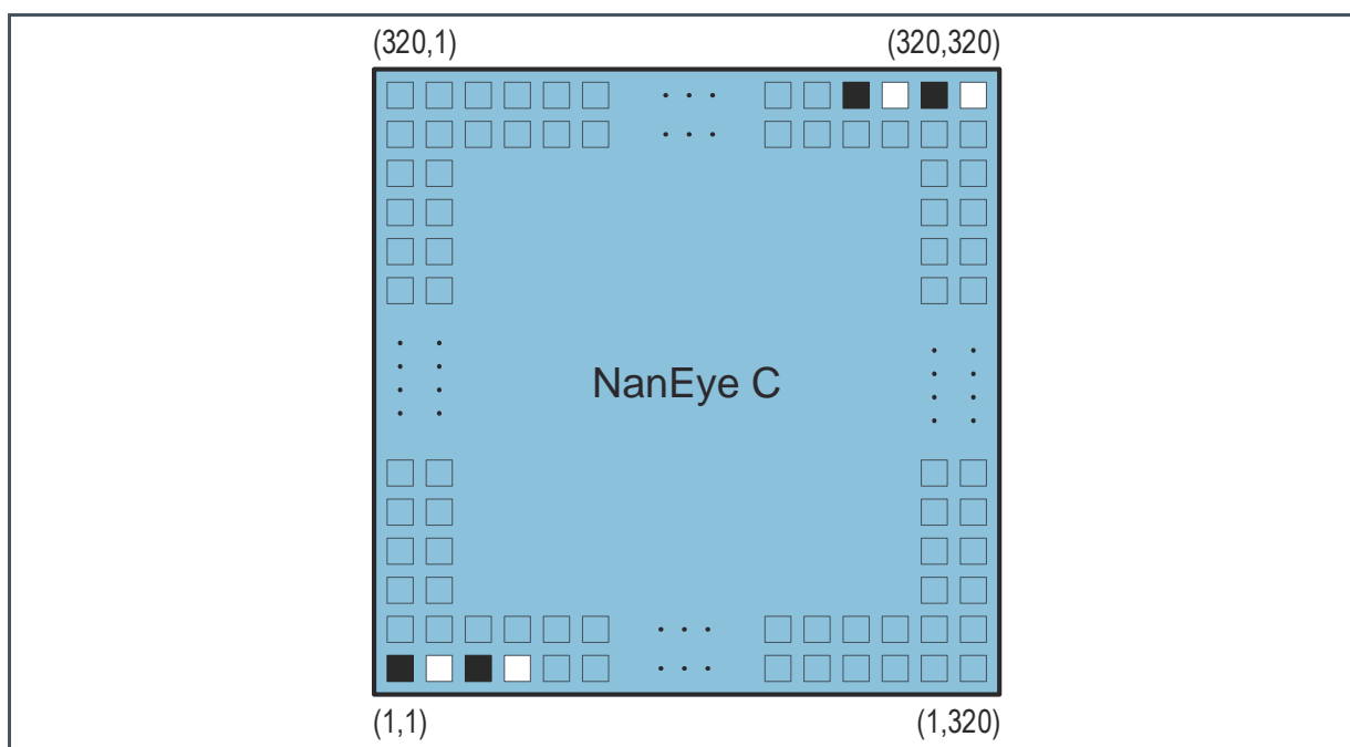
Figure 13 : Pixel Array
