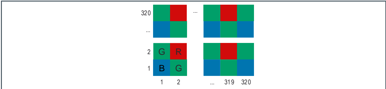
Figure 15: Colored Version Bayer Pattern Matrix
