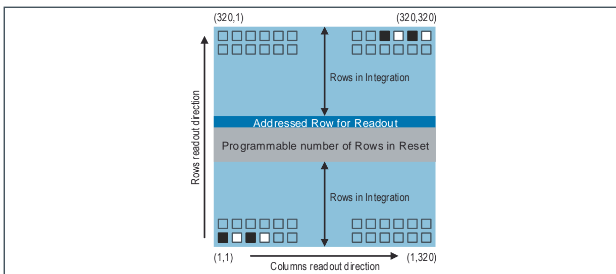
Figure 32: Row Readout Operation
