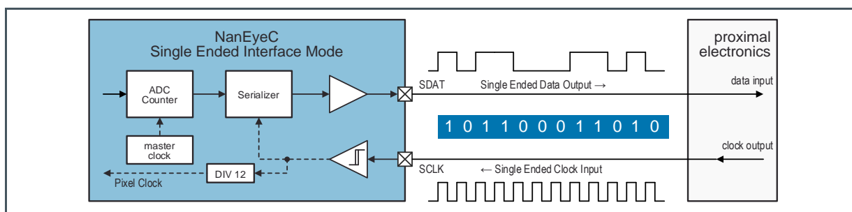
Figure 25 : SEIM Downstream
