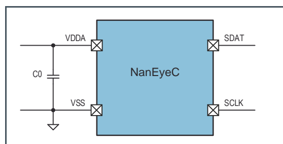
Figure 41: External Components SEIM
