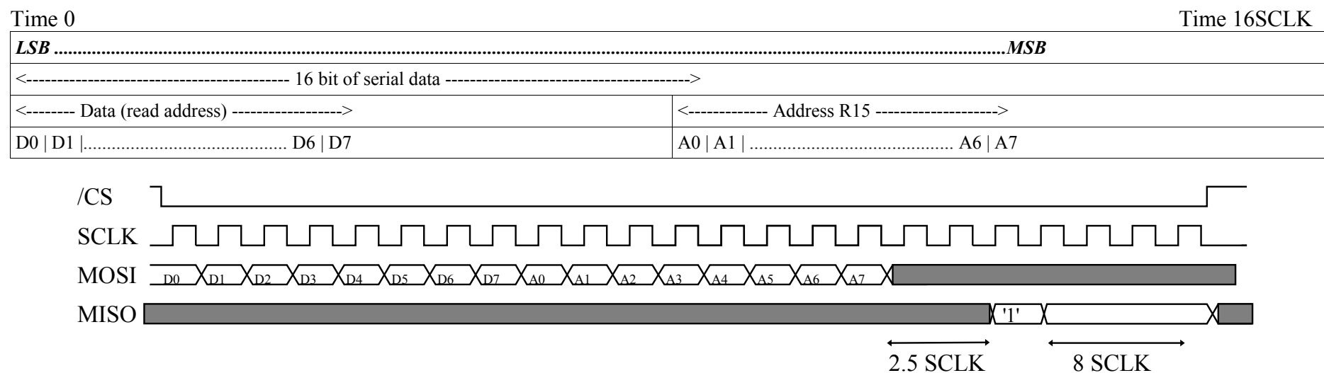
Fig 19: Reading operation
