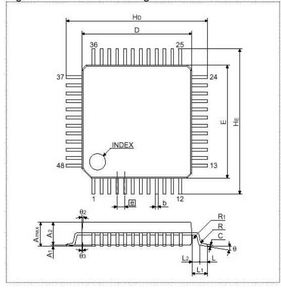
Figure 7: TQFP48 Package
