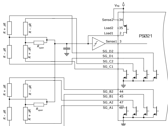
Figure 16: 2 Fullbridges
