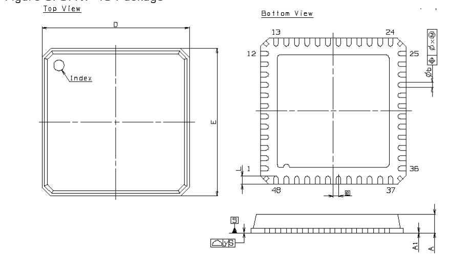
Figure 8: QFN7-48 Package
