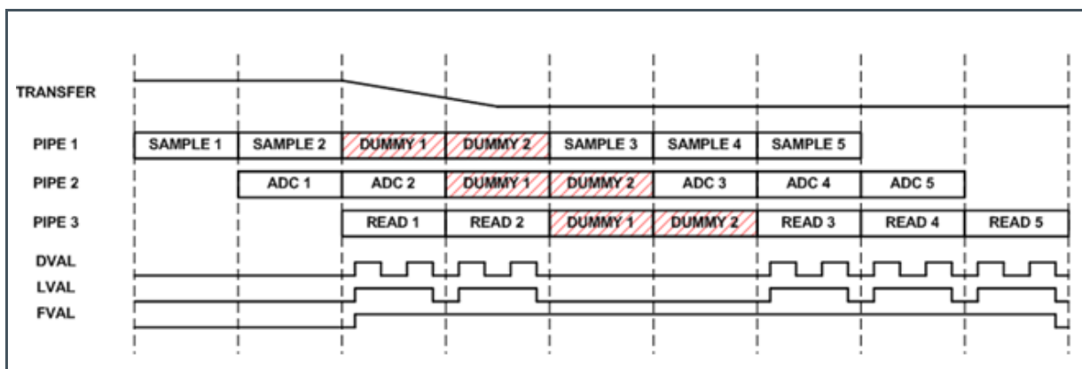
Figure 87: Timing of DVAL, LVAL and FVAL to Avoid Horizontal Line Artifact
