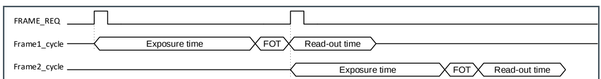
Figure 29: Two Requests for 1 Frame in Internal Exposure Mode (1)
