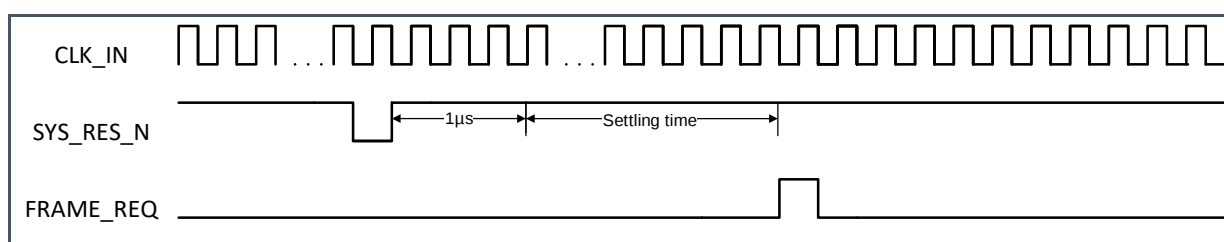
Figure 23: Reset Sequence
