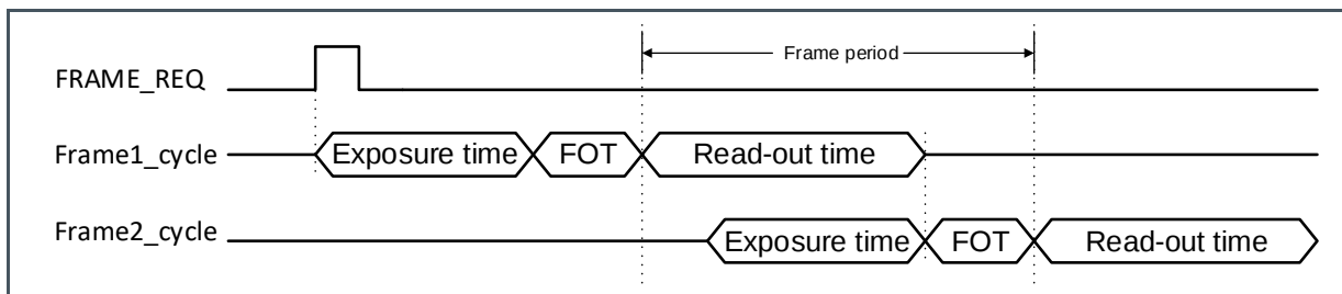
Figure 20: Frame Period
