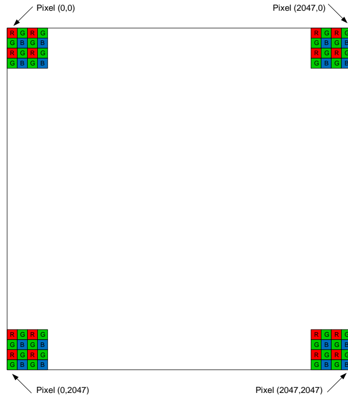
Figure 52: RGB Bayer pattern order
