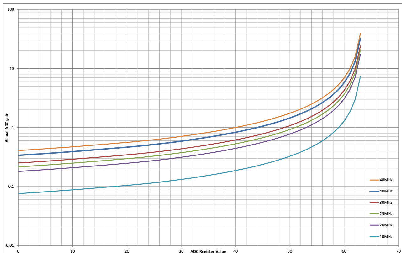
Figure 43: Actual ADC gain vs. ADC register value [103]
