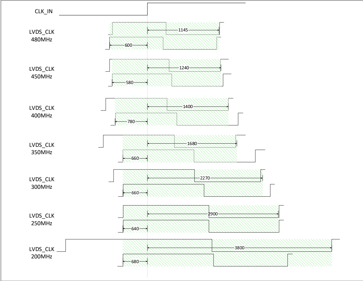
Figure 15: LVDS clock delay versus master clock
