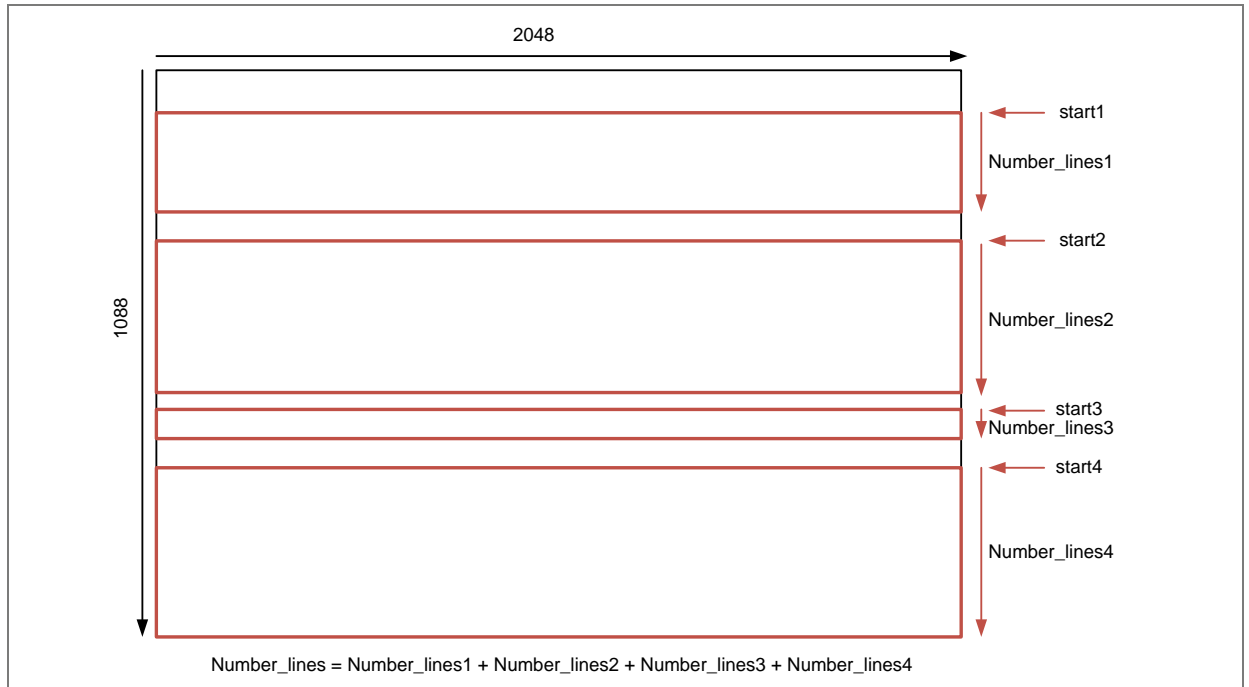
Figure 51: Example of 4 multiple frames read-out
