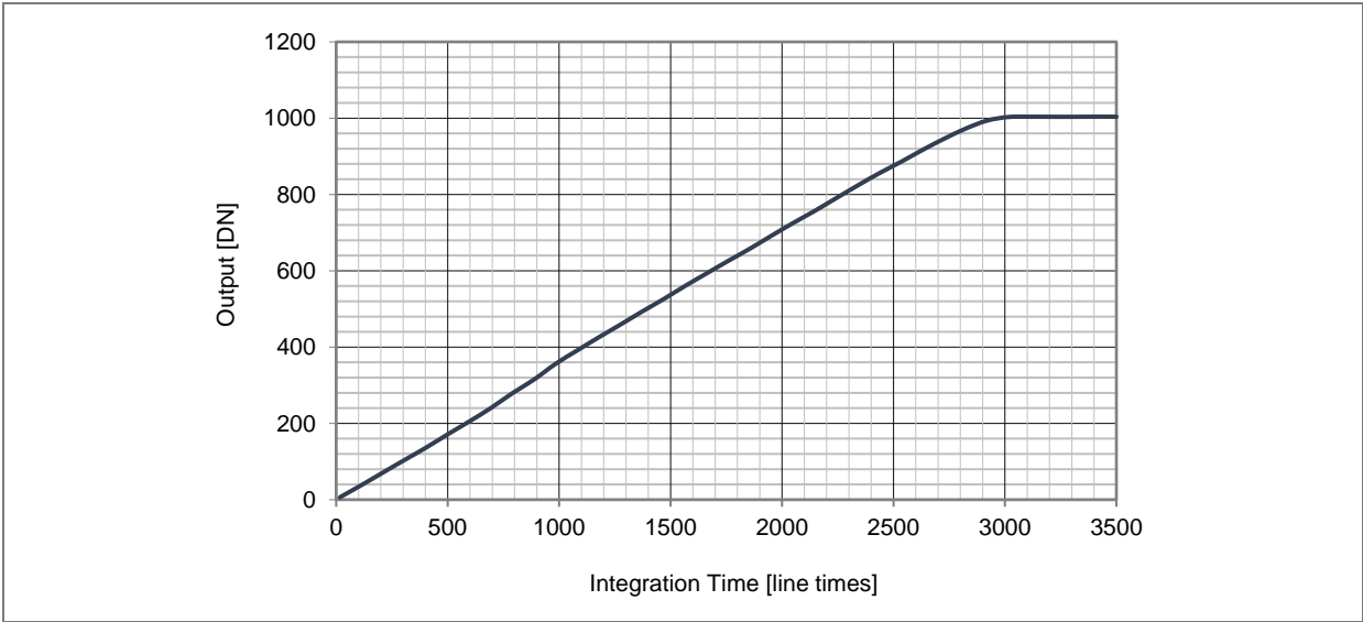
Figure 59: Typical response curve
