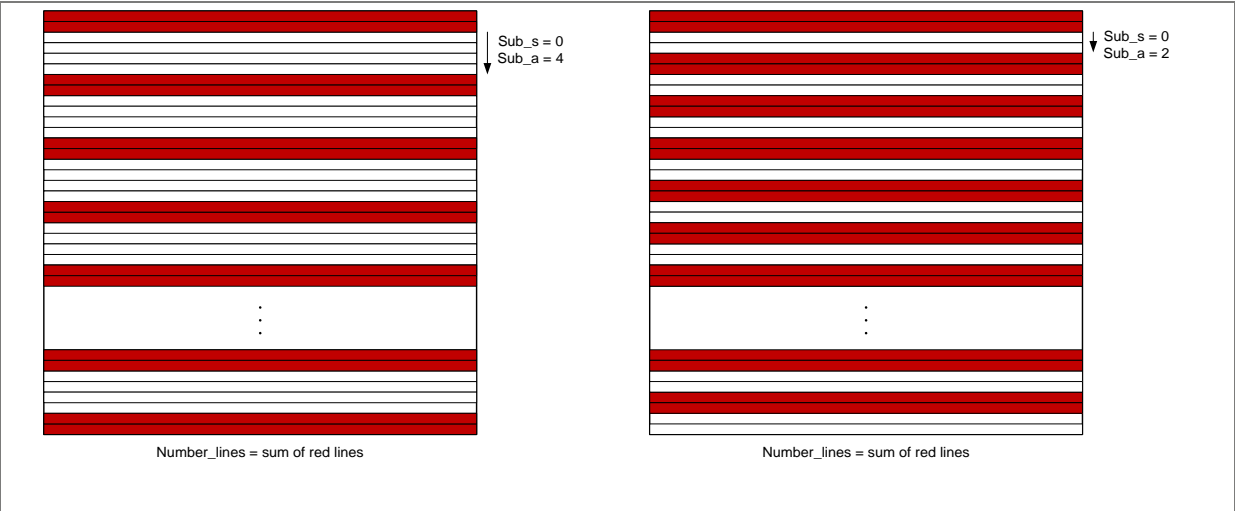
Figure 54: Subsampling examples in advanced mode (skip 4x and skip 2x)
