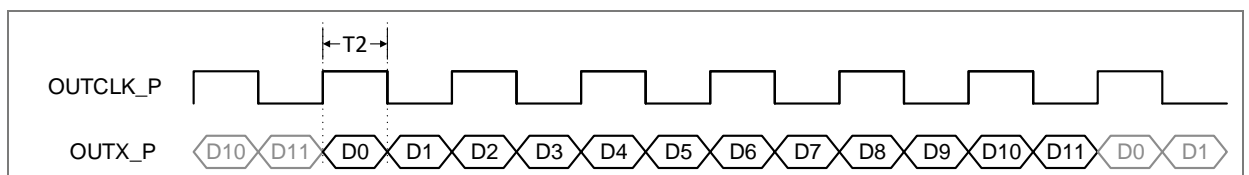
Figure 31: 12-bit pixel data on an LVDS channel
