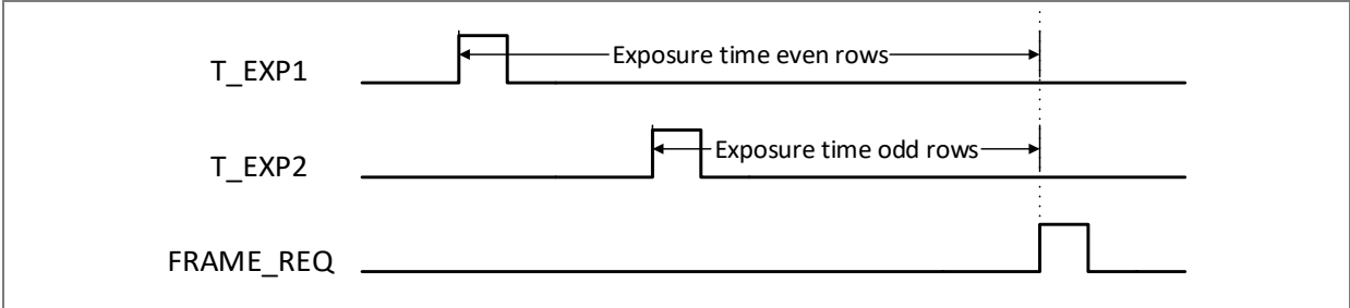
Figure 46: Interleaved read-out in external exposure mode
