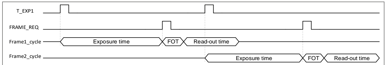
Figure 29: Request for 2 frames using external-Exposure-time mode
