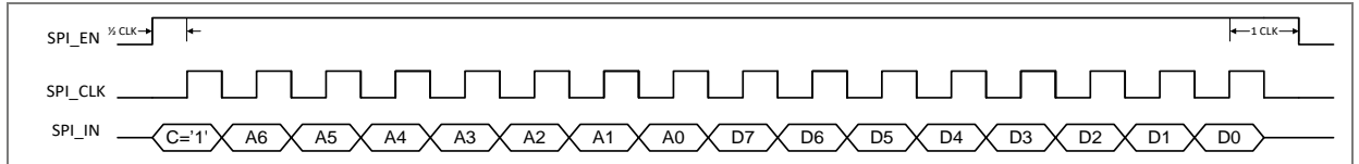
Figure 21: SPI write timing
