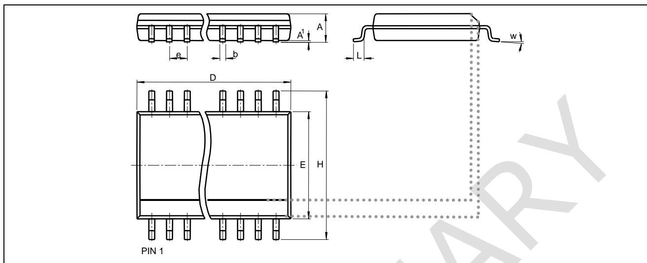
Figure 2: Shape &amp; Dimensions
