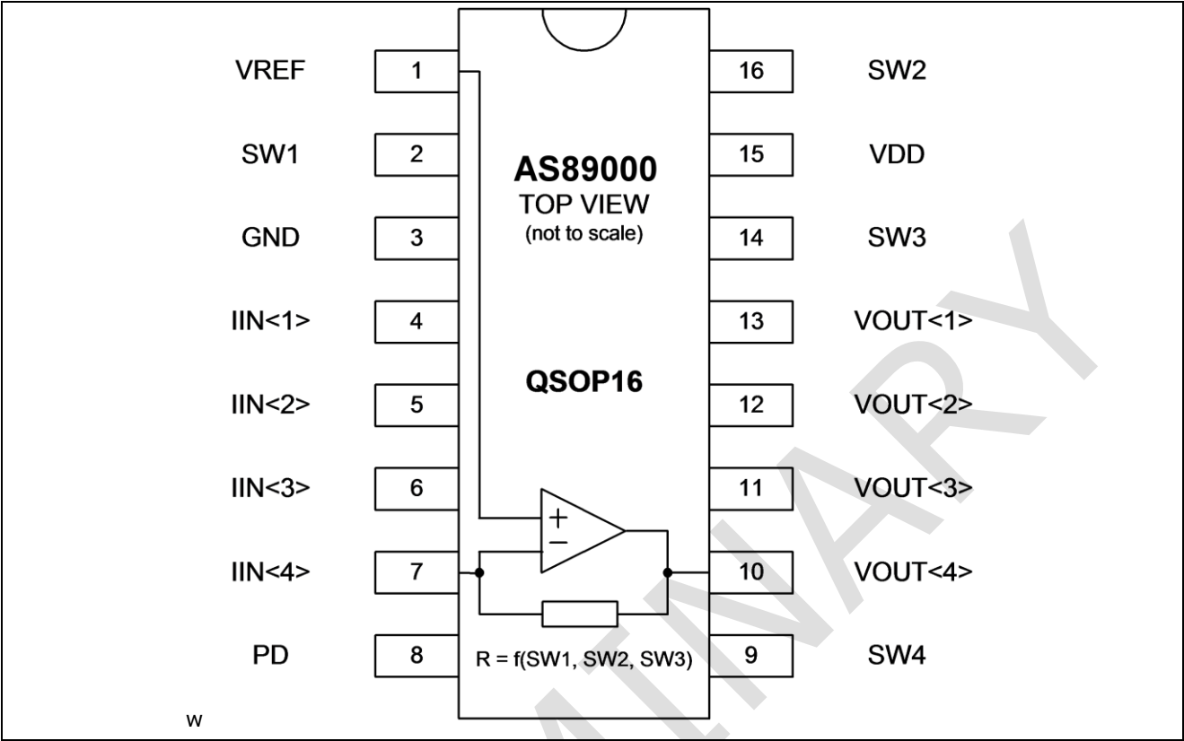
Figure 3: Pin Configuration
