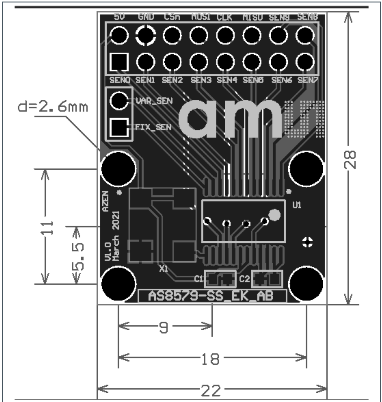
Figure 9: PCB Layout
