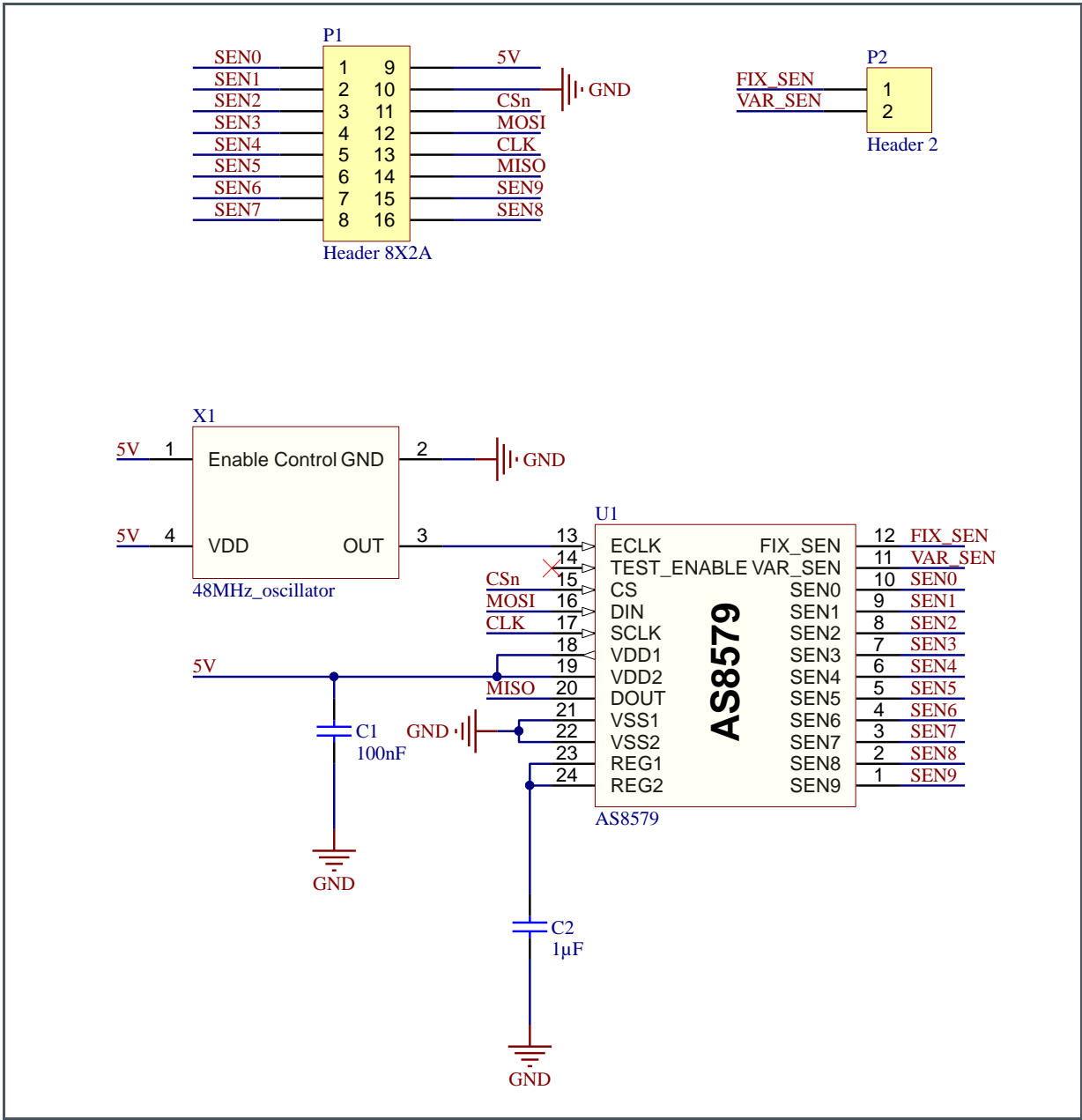
Figure 8: Schematic
