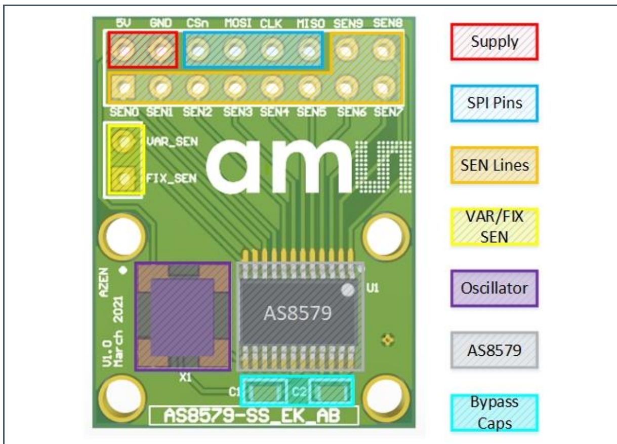
Figure 4: AS8579 Adapter Board Overview
