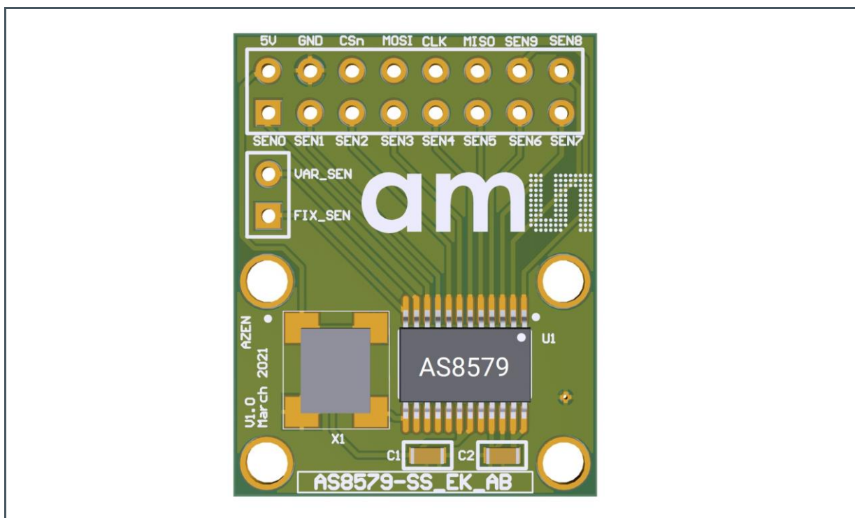
Figure 2: AS8579 Adapter Board
