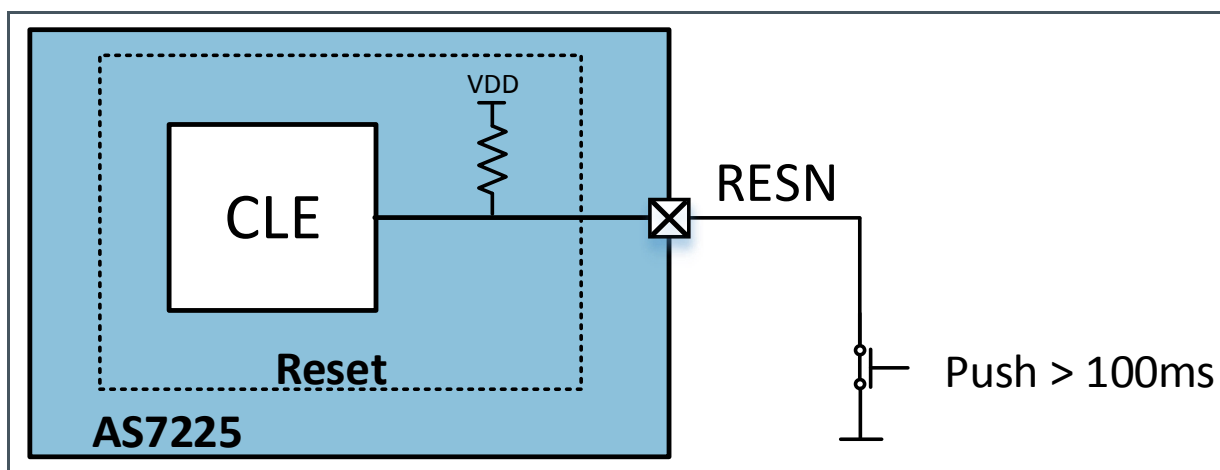
Figure 12: Reset Circuit
