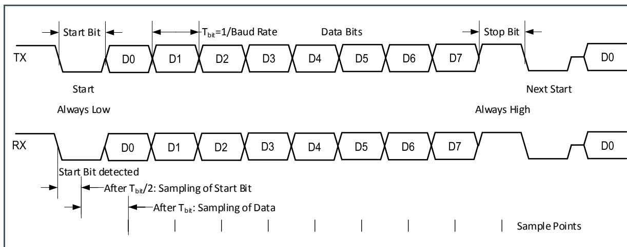
Figure 79: UART Protocol
