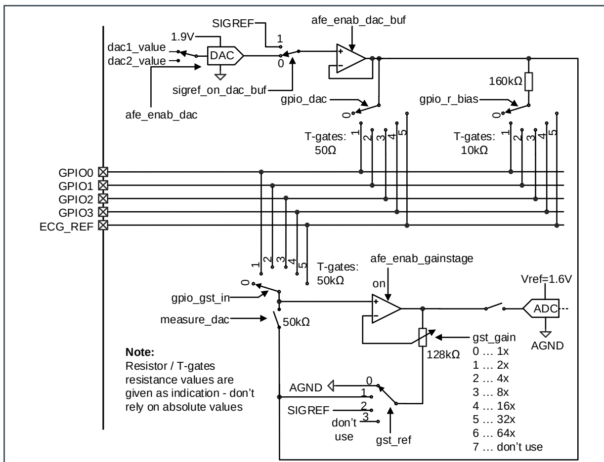
Figure 103: AFE Schematic
