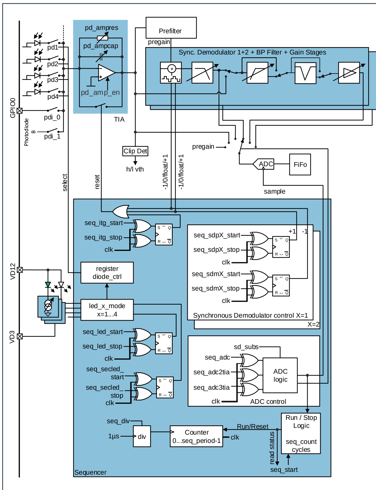
Figure 41: Block Diagram of Sequencer
