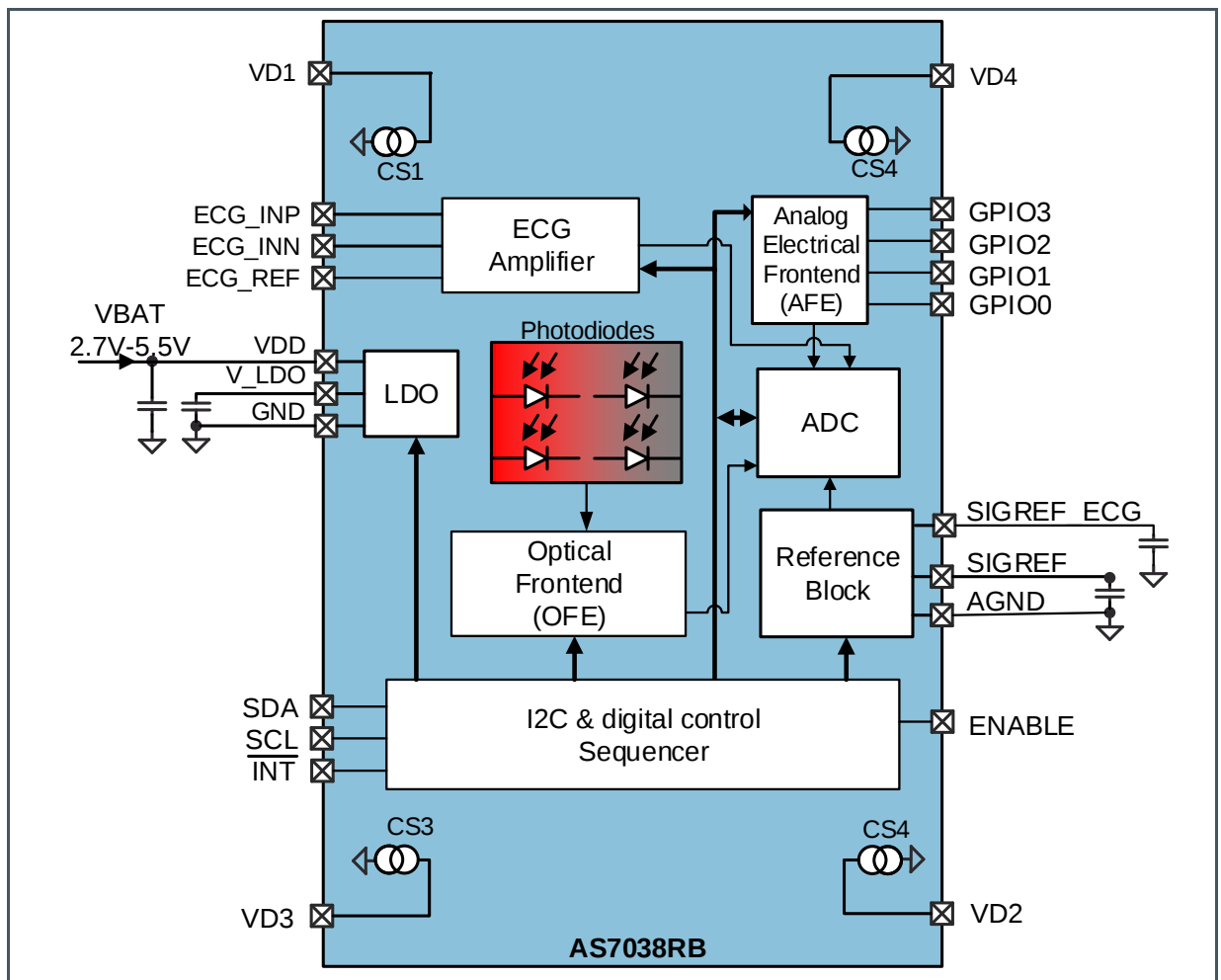
Figure 2 : Functional Blocks of AS7038RB
