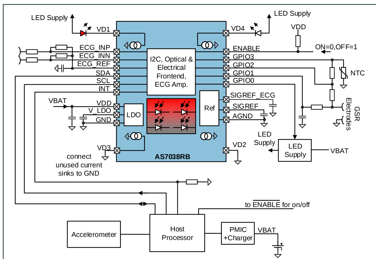
Figure 170: AS7038RB Optical SpO2 and HRM Measurement System for Wrist Based Application
