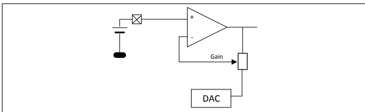
Figure 117: Non Inverting Amplifier High Impedance, GND Referenced
