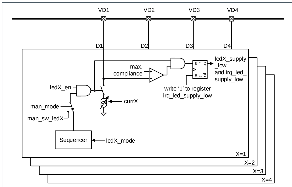
Figure 10: LED Drivers
