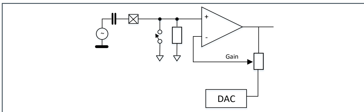
Figure 101: Non Inverting Amplifier with DC-Blocking and Fast Settling Time, Referenced to \text{ADCRef} / 2
