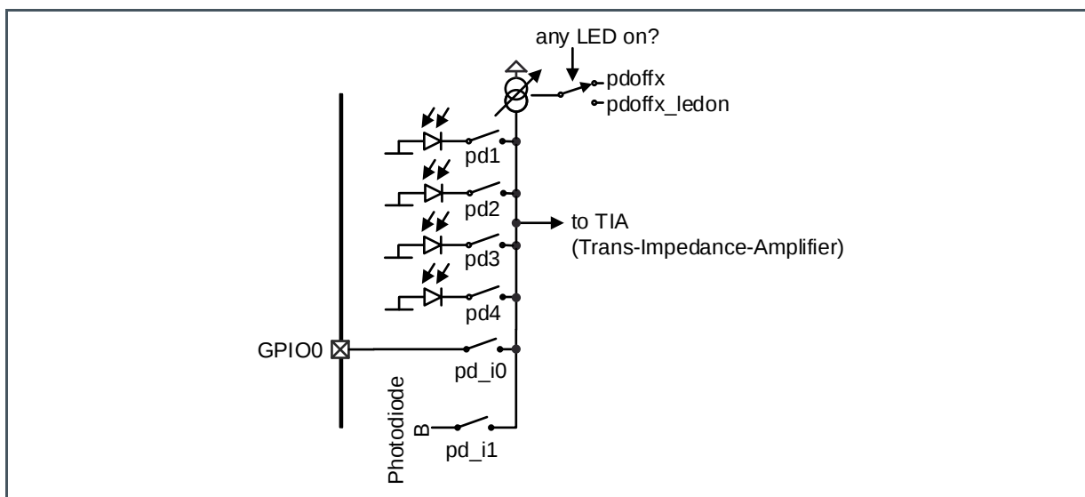
Figure 21: Photodiode Selection
