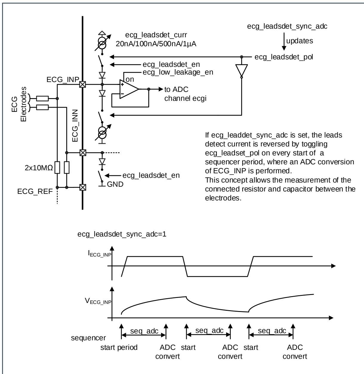
Figure 103: ECG Lead OFF Detection Internal Circuit
