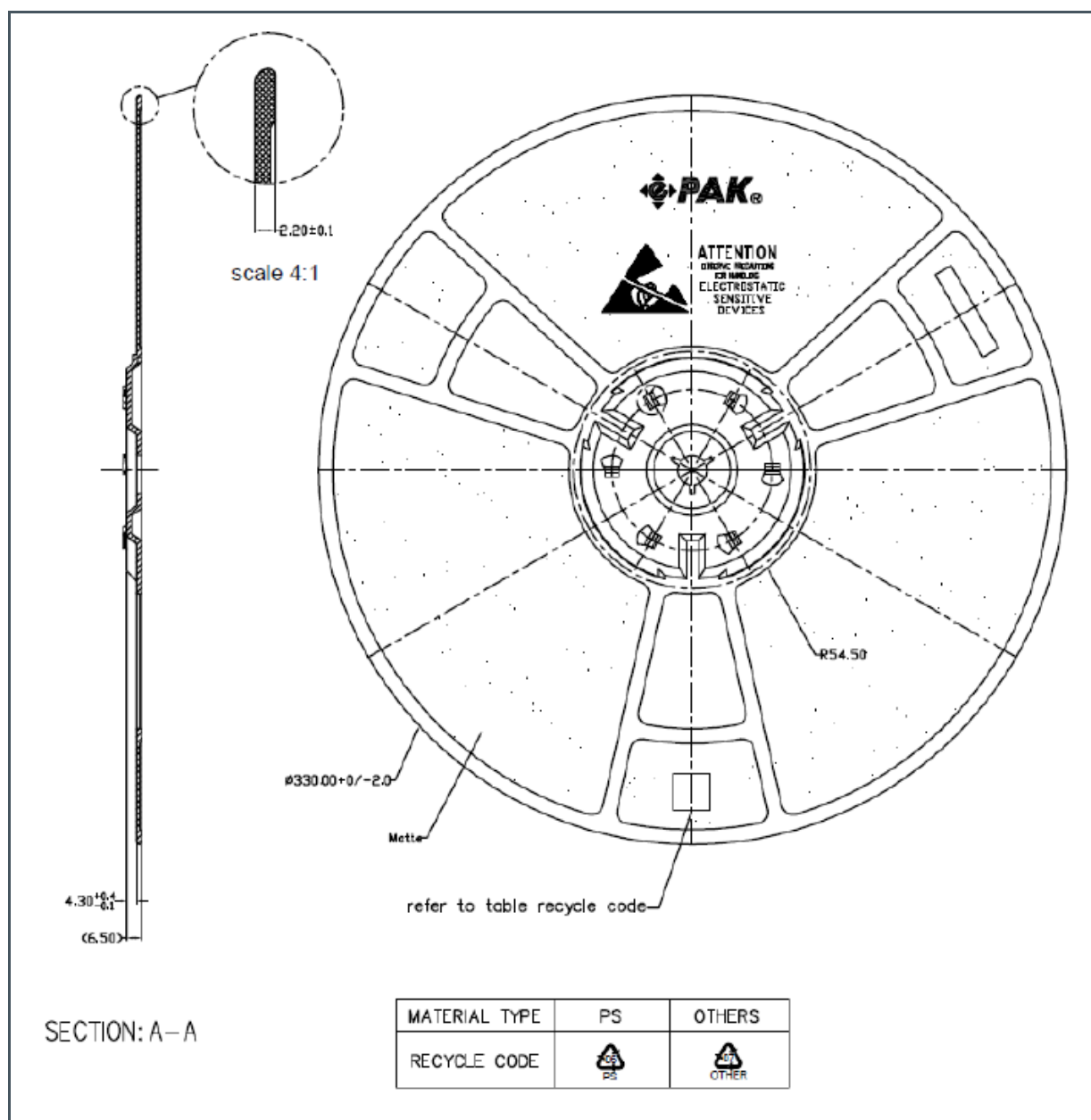
Figure 147: AS7026GG Reel Dimensions
