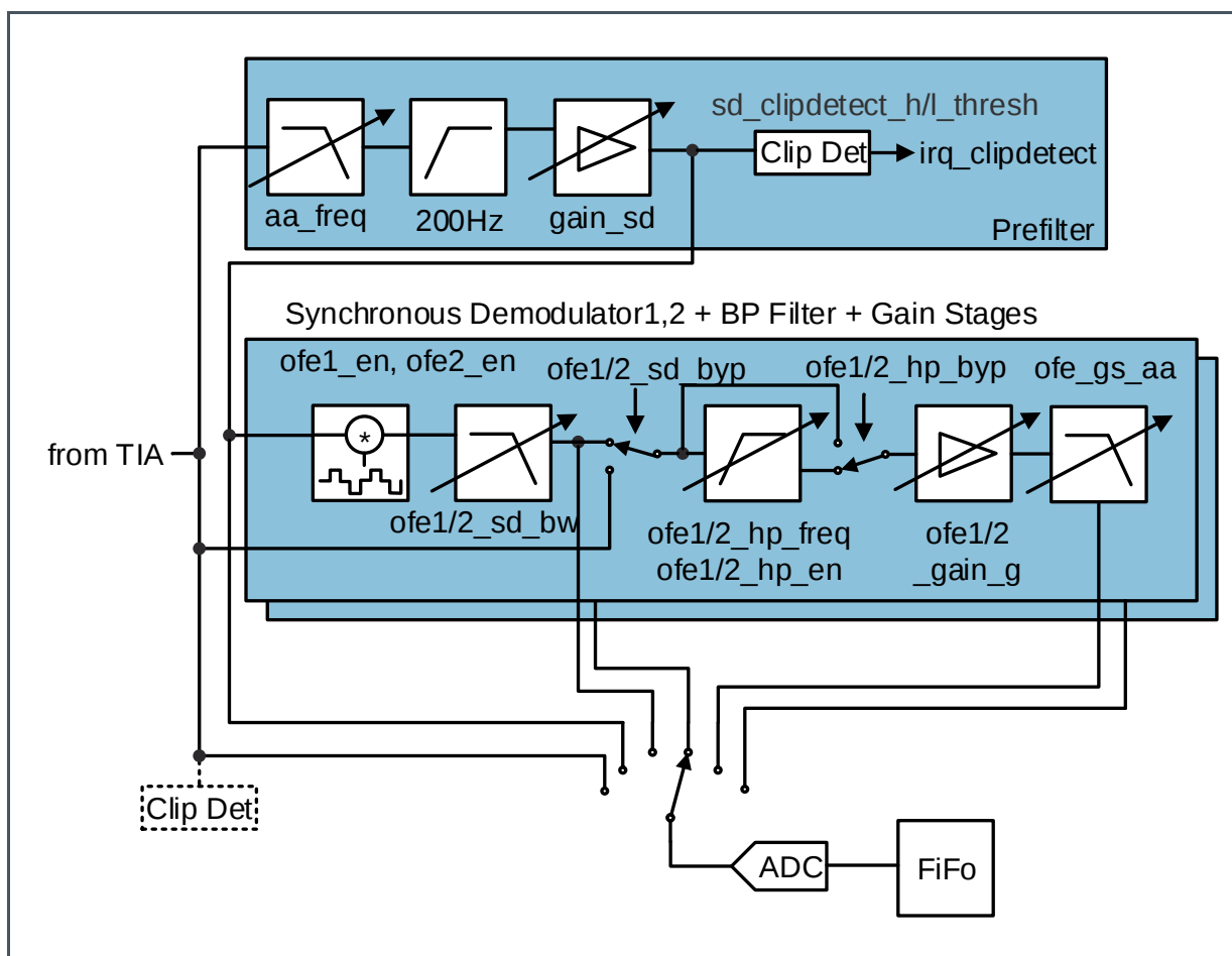
Figure 63: Optical Signal Conditioning
