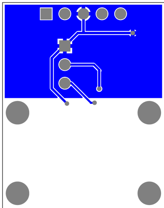
Figure 6: Bottom Layer
