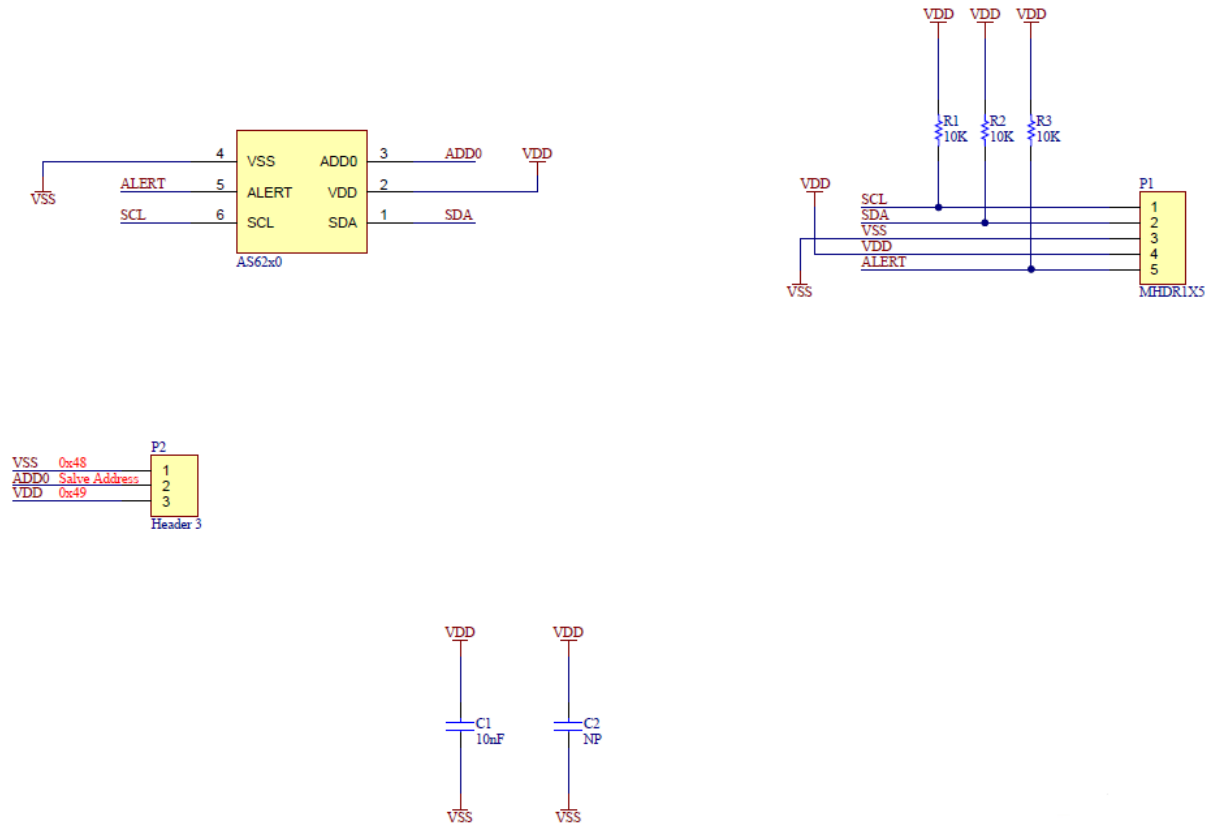
Figure 4: Schematics
