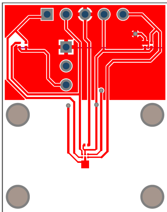
Figure 5: Top Layer
