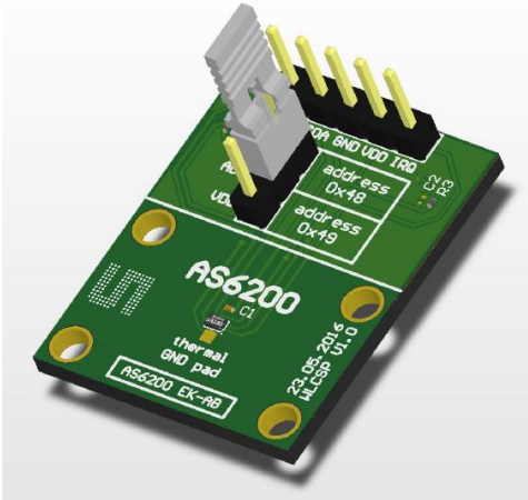
Figure 1: adapter board
