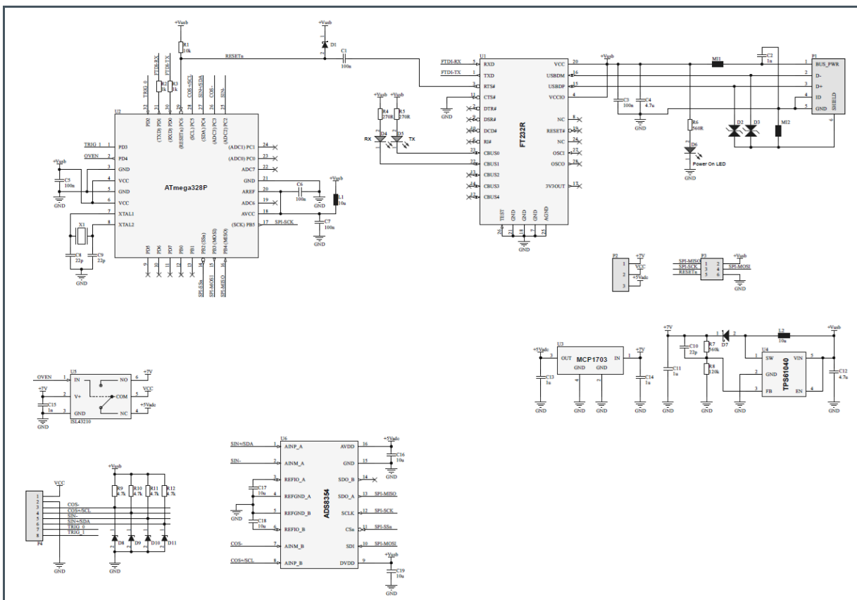
Figure 7: AS5715_BP_x.x Schematic
