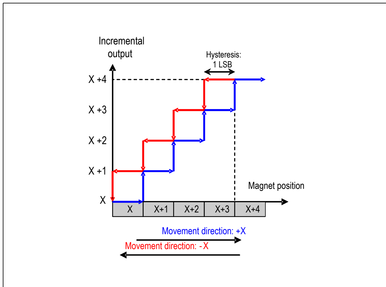
Figure 15: Hysteresis of the Incremental Output
