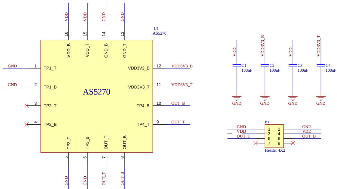
Figure 3: AS5270-MF_EK_SB schematics
