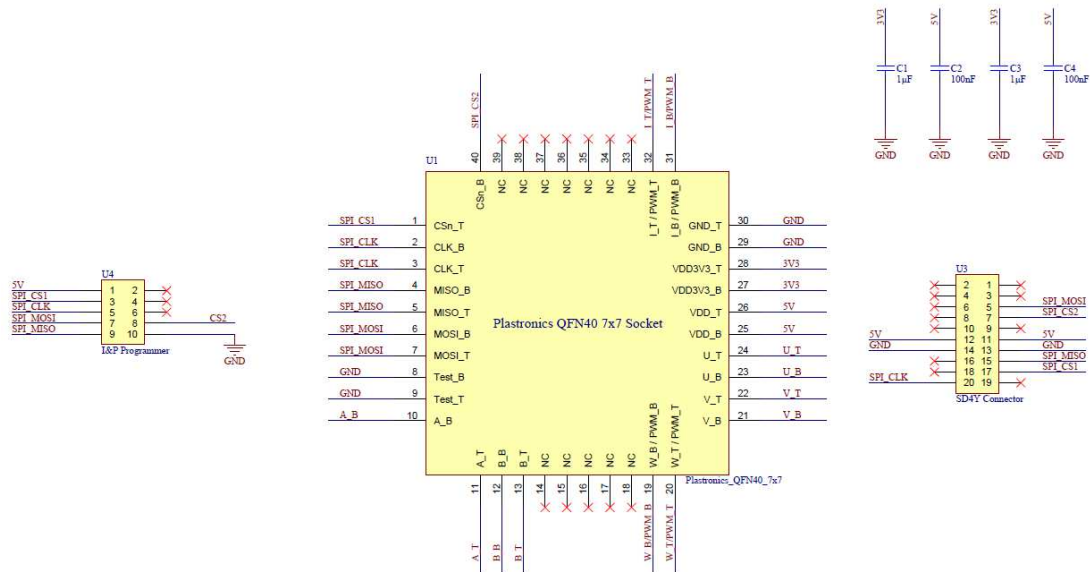
Figure 4: AS5247-MF_EK_SB schematics
