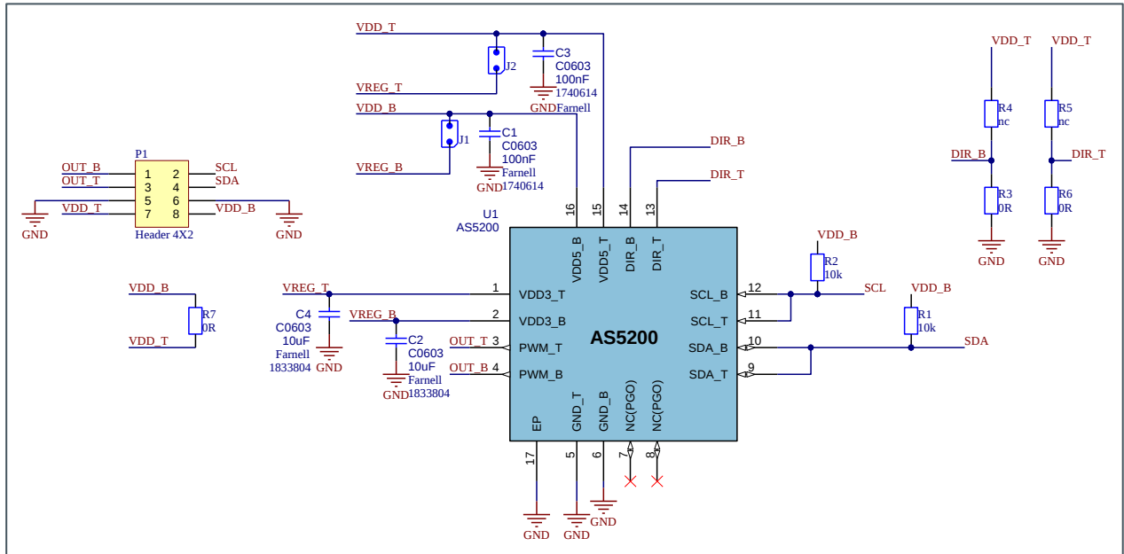
Figure 6: AS5200L-MF_EK_AB schematics
