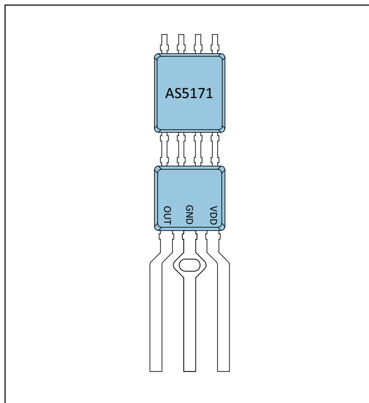
Figure 5: AS5171A/B Pin Assignment (Top View, SIP)
