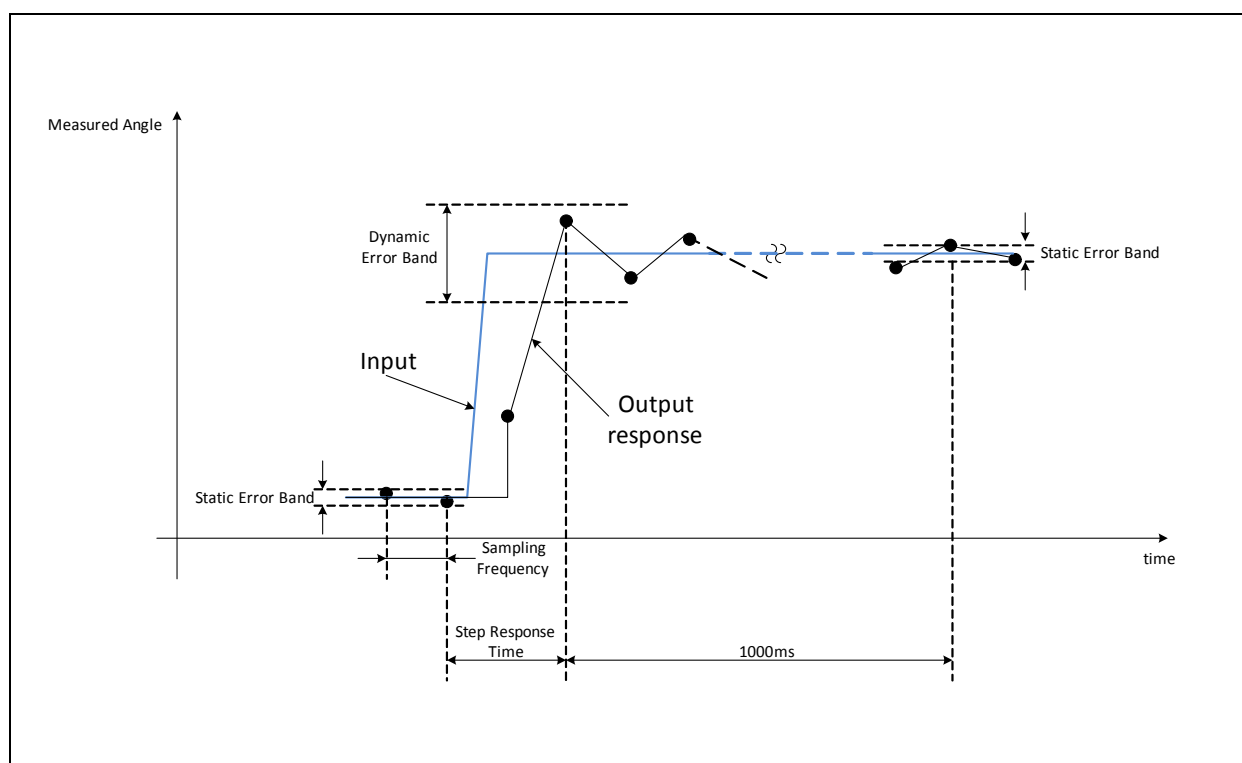
Figure 26: Step Response
