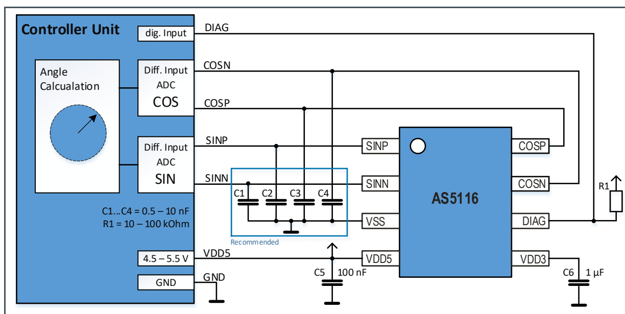
Figure 28: AS5116 Minimum Wiring Diagram, Differential Output Mode
