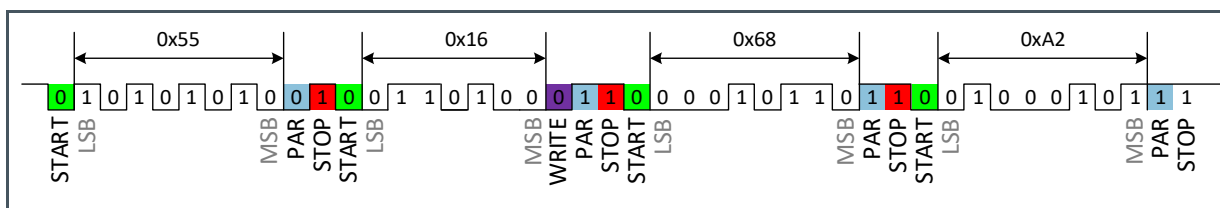
Figure 15: UART – Write Example
