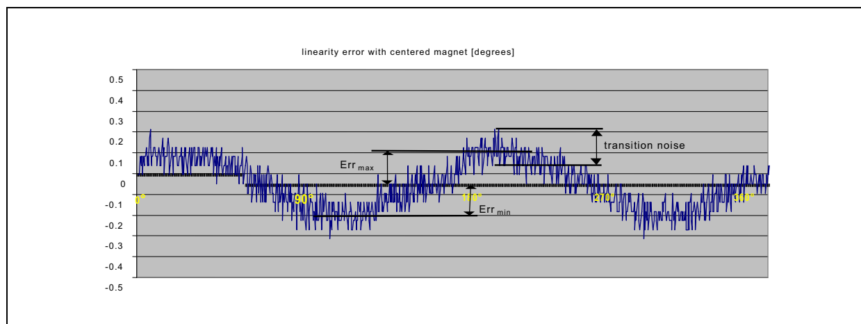
Figure 26: Example of Linearity Error Over 360°
