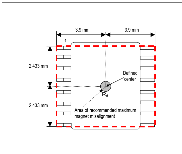
Figure 23: Defined IC Center and Magnet Displacement Radius
