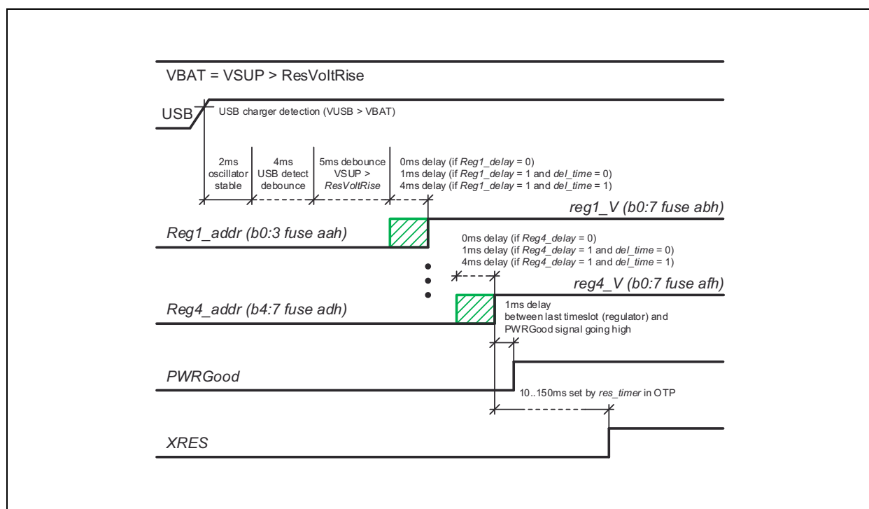
Figure 44: Start-Up Sequence Diagram 3/5
