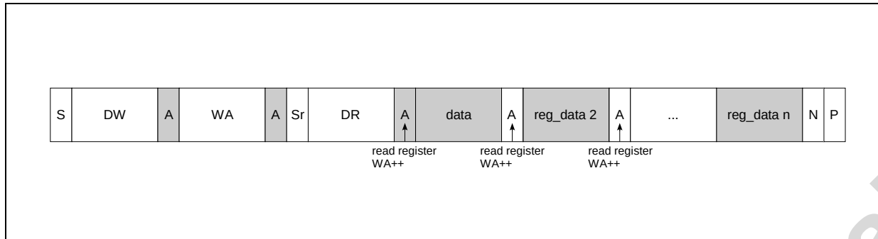
Figure 18. Sequential Read
