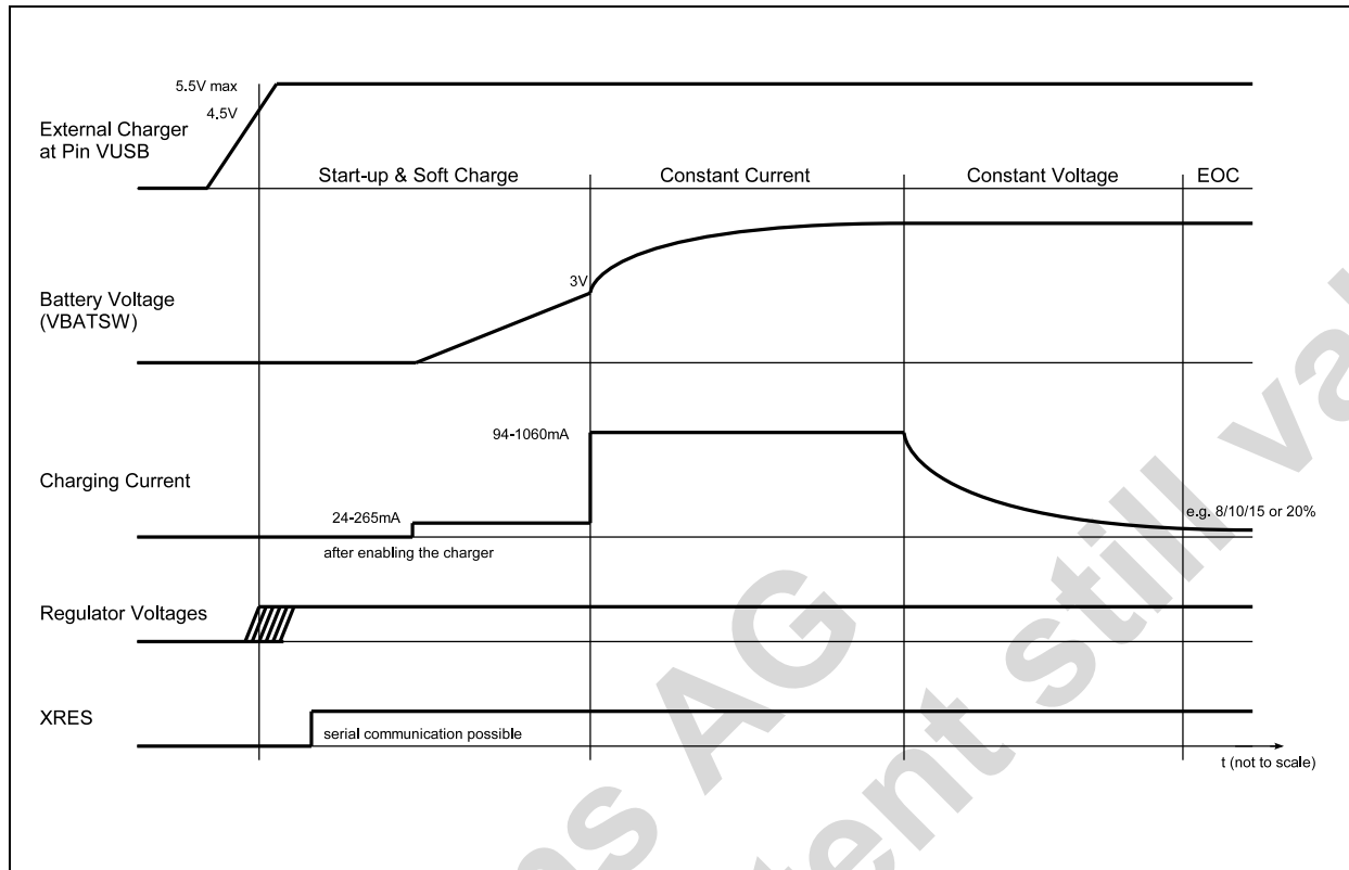
Figure 13. Charger States
