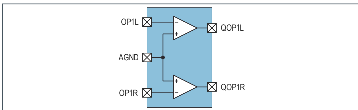
Figure 33: Operational Amplifier
