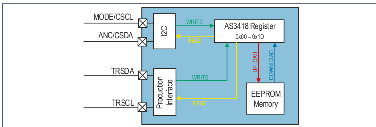
Figure 52: Register Access
