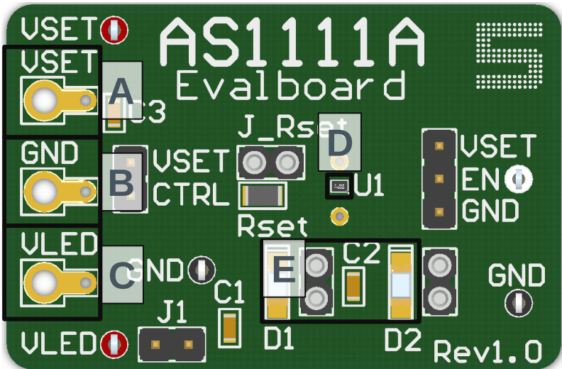
Figure 2: Evaluation Board Overview
