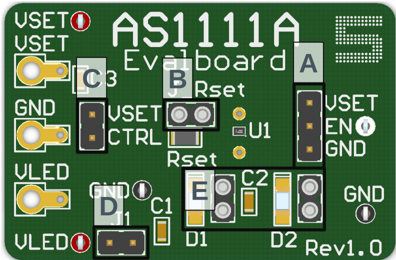
Figure 3: Jumper and device locations
